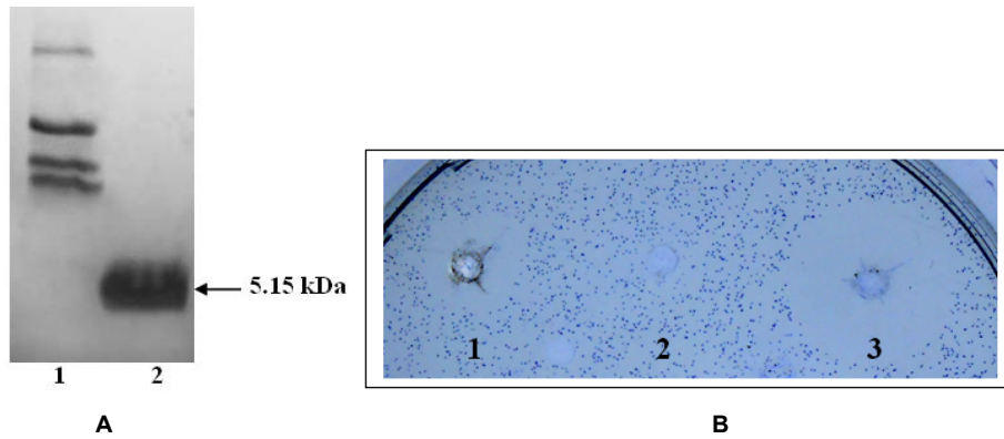
Fig. 2. A. SDS-PAGE analysis of rec-hBD-3 purified by reverse phase chromatography on Sep-Pak C18 (Water, USA).
