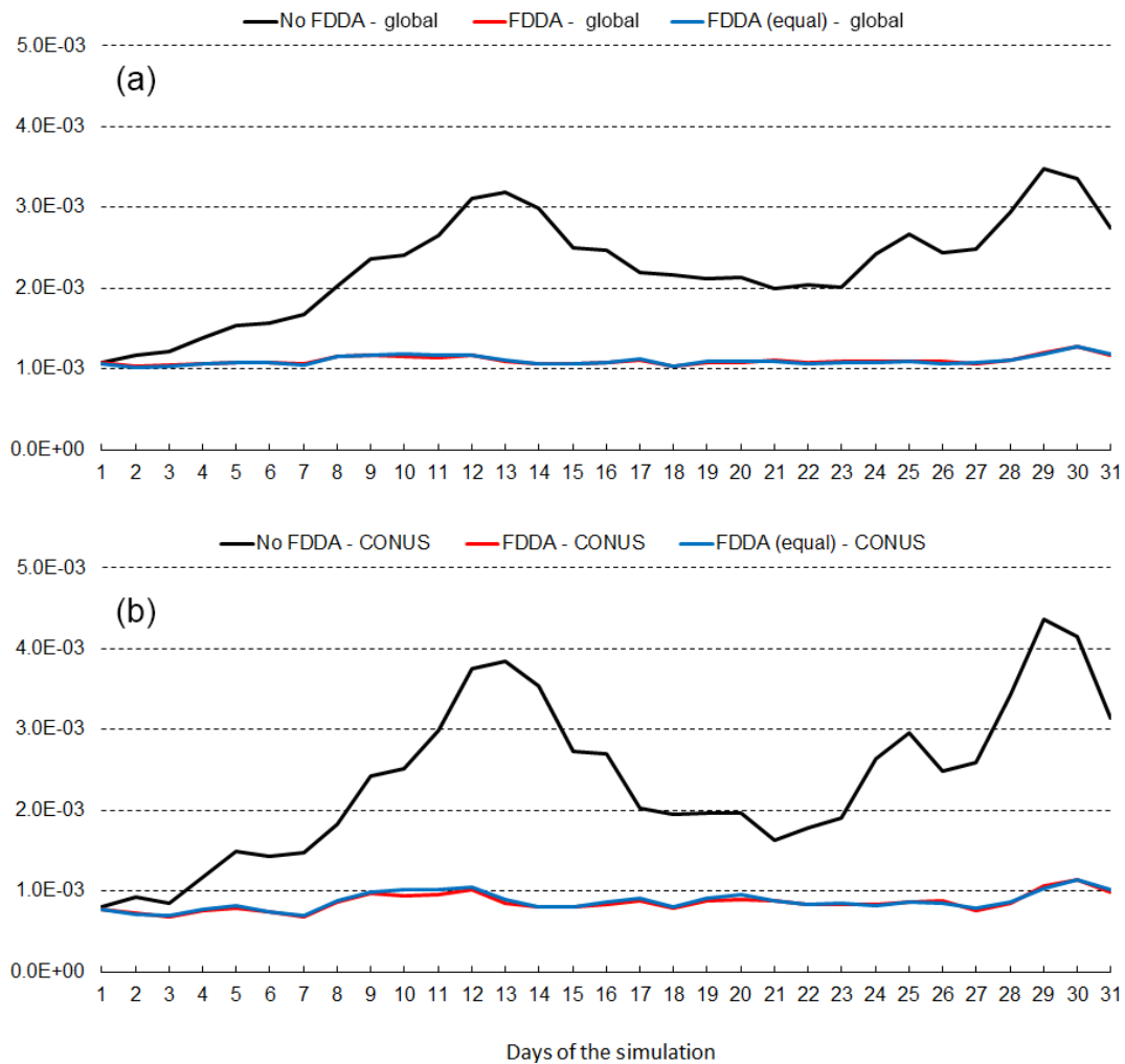
Figure 14. January 2013 time series plots of 2 m water vapor mixing ratio ( q_v ) RMSE for MPAS-A without FDDA (black line), MPAS-A with FDDA applied using weaker q_v nudging (red line), and MPAS-A with FDDA applied at equal strength for all variables (blue line). Panel (a) shows results for the entire global domain, while (b) shows results for the CONUS subdomain.
