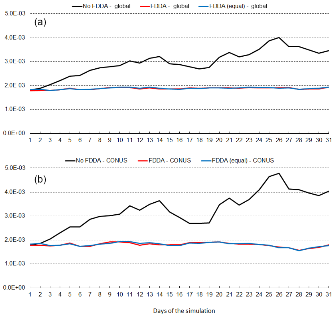
Figure 15. July 2013 time series plots of 2 m water vapor mixing ratio ( q_v ) RMSE for MPAS-A without FDDA (black line), MPAS-A with FDDA applied using weaker q_v nudging (red line), and MPAS-A with FDDA applied at equal strength for all variables (blue line). Panel (a) shows results for the entire global domain, while (b) shows results for the CONUS subdomain.
