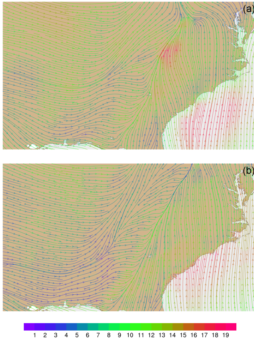
Figure 11. Streamline analysis for layer 1 (surface) at 00:00 UTC on 31 January 2013 focused on the southeastern United States (a) from MPAS-A using FDDA and (b) FDDA target field. Streamline color indicates wind speed ( \text{m s}^{-1} ).
