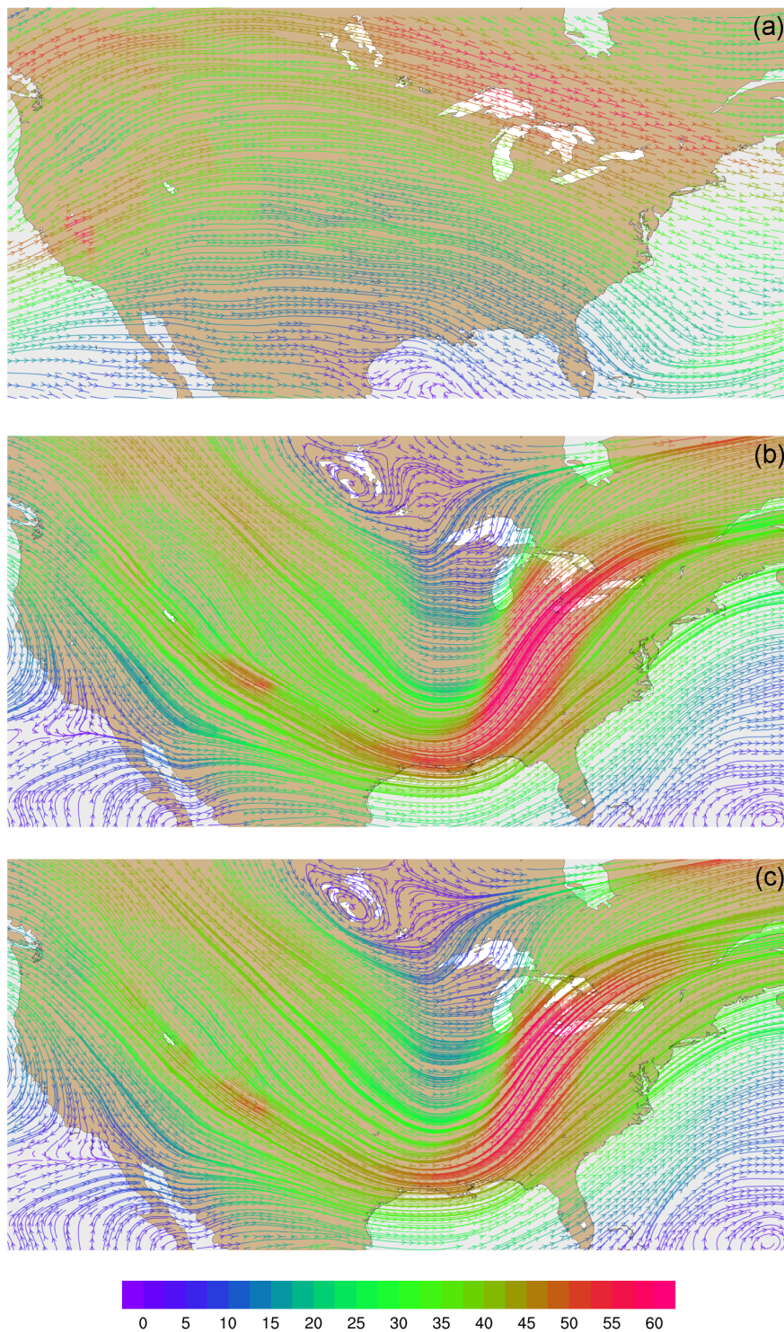
Figure 10. Streamline analyses for layer 28 ( \sim 500\text{--}300 hPa) at 00:00 UTC on 31 January 2013 focused on the contiguous United States (a) from MPAS-A without FDDA, (b) FDDA target field, and (c) MPAS-A using FDDA. Streamline color indicates wind speed ( \text{m s}^{-1} ).
