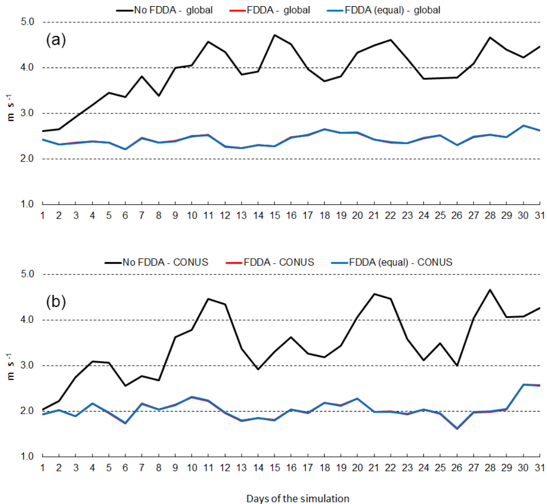
Figure 16. January 2013 time series plots of 10 m wind speed RMSE for MPAS-A without FDDA (black line), MPAS-A with FDDA applied using weaker q_v nudging (red line), and MPAS-A with FDDA applied at equal strength for all variables (blue line). Panel (a) shows results for the entire global domain, while (b) shows results for the CONUS subdomain.
