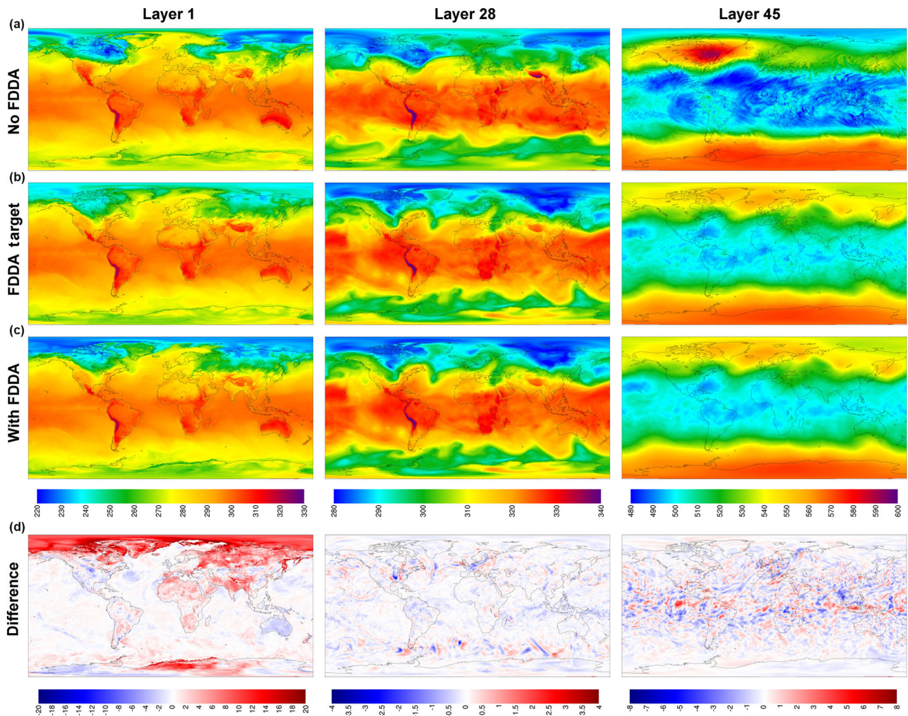
Figure 3. MPAS-A simulation results without FDDA (a), FDDA target fields (b), MPAS-A results with FDDA (c), and FDDA target minus MPAS-A with FDDA (d) for potential temperature (K) in layers 1, 28, and 45, for 00:00 UTC on 31 January 2013, 30 days into the simulation.
