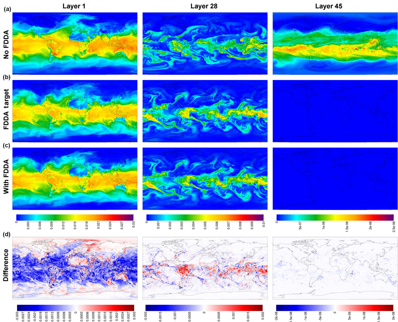
Figure 6. MPAS-A simulation results without FDDA (a), FDDA target fields (b), MPAS-A results with FDDA (c), and FDDA target minus MPAS-A with FDDA (d) for water vapor mixing ratio ( \text{kg kg}^{-1} ) in layers 1, 28, and 45, for 00:00 UTC on 31 January 2013, 30 days into the simulation.
