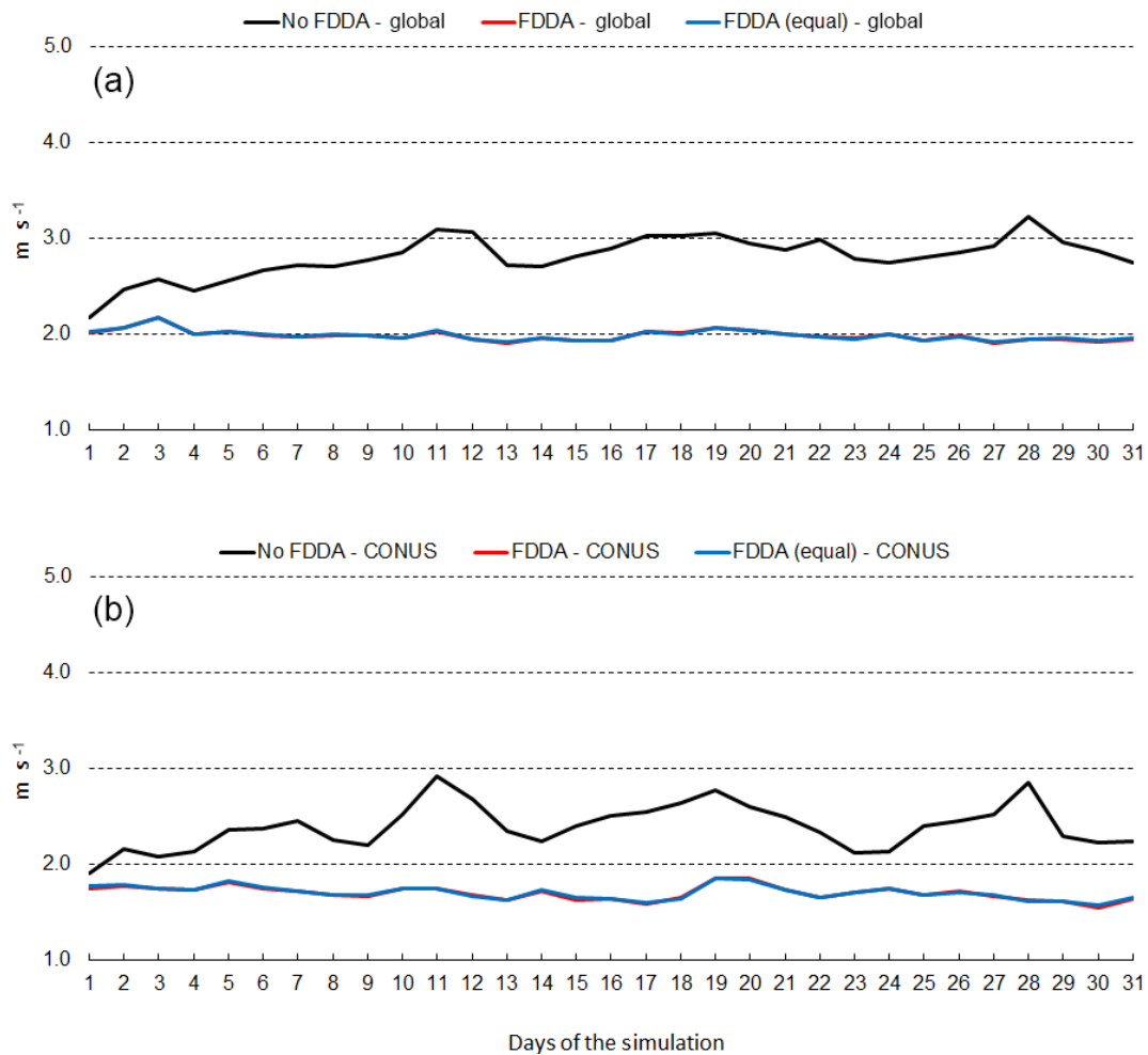
Figure 17. July 2013 time series plots of 10 m wind speed RMSE for MPAS-A without FDDA (black line), MPAS-A with FDDA applied using weaker q_v nudging (red line), and MPAS-A with FDDA applied at equal strength for all variables (blue line). Panel (a) shows results for the entire global domain, while (b) shows results for the CONUS subdomain.
