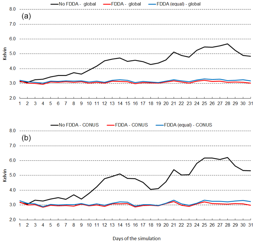
Figure 13. July 2013 time series plots of 2 m temperature RMSE for MPAS-A without FDDA (black line), MPAS-A with FDDA applied using weaker q_v nudging (red line), and MPAS-A with FDDA applied at equal strength for all variables (blue line). Panel (a) shows results for the entire global domain, while (b) shows results for the CONUS subdomain.
