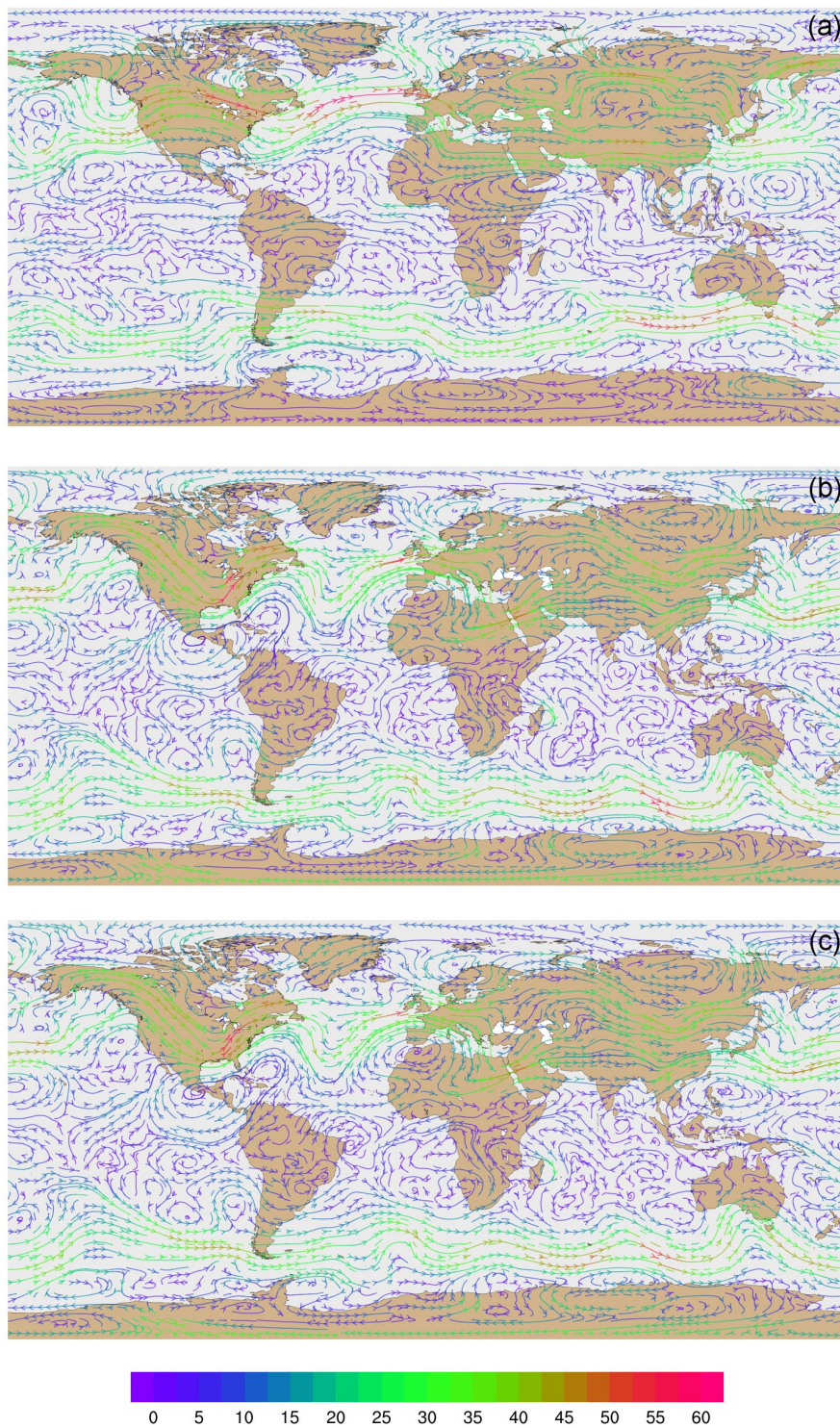
Figure 9. Global streamline analyses for layer 28 (~500–300 hPa) at 00:00 UTC on 31 January 2013 (a) from MPAS-A without FDDA, (b) FDDA target field, and (c) MPAS-A using FDDA. Streamline color indicates wind speed ( \text{m s}^{-1} ).
