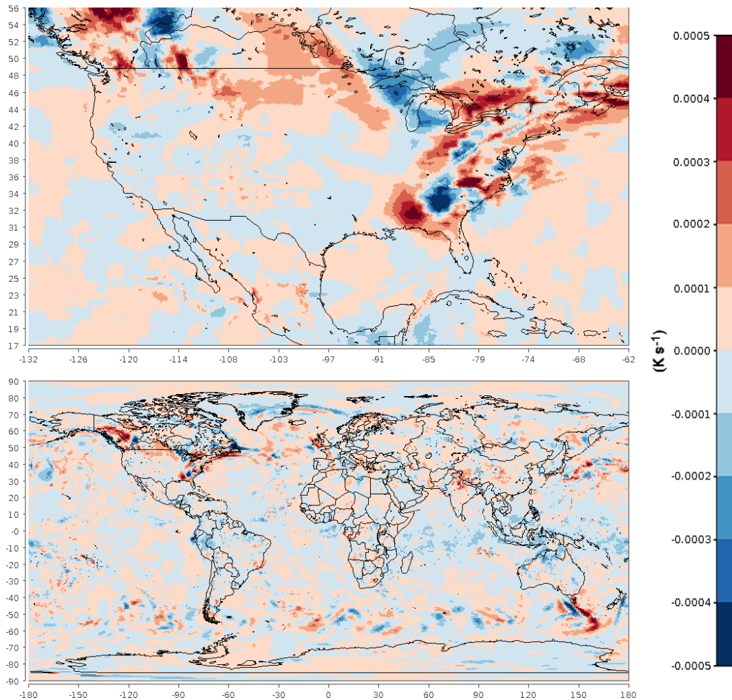
Figure 5. Spatial plots of the nudging term for potential temperature in layer 28 at 00:00 UTC on 18 January 2013.
