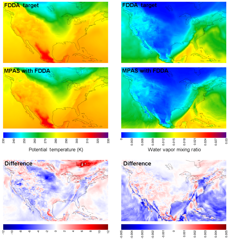
Figure 7. Simulation results from MPAS-A using FDDA and FDDA target fields for potential temperature (K) and water vapor mixing ratio ( \text{kg kg}^{-1} ) in layer 1 at 00:00 UTC on 31 January 2013 focused on the contiguous United States. The difference fields indicate FDDA target minus MPAS-A with FDDA to match the polarity of nudging.
