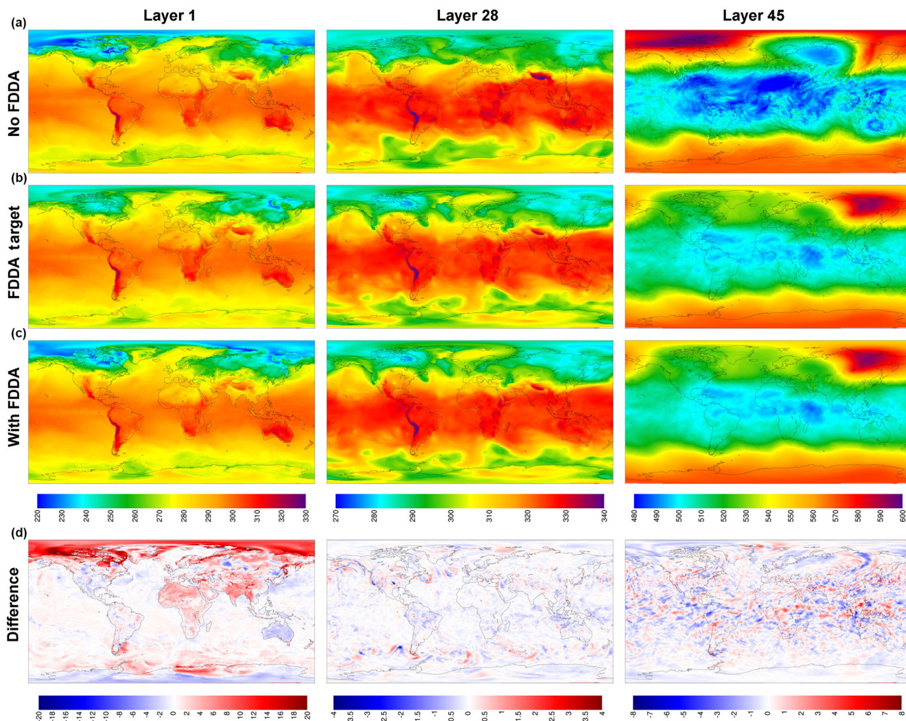
Figure 2. MPAS-A simulation results without FDDA (a), FDDA target fields (b), MPAS-A results with FDDA (c), and FDDA target minus MPAS-A with FDDA (d) for potential temperature (K) in layers 1, 28, and 45, for 00:00 UTC on 11 January 2013, 10 days into the simulation.
