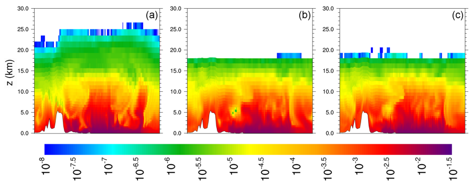
Figure 8. Cross-sectional plots of water vapor mixing ratio ( \text{kg kg}^{-1} ) along longitude 80^\circ \text{E} from 55^\circ \text{N} to 55^\circ \text{S} for 00:00 UTC on 31 January 2013 (a) from MPAS-A without FDDA, (b) FDDA target field, and (c) MPAS-A using FDDA at 1/10 the strength compared to the other nudged variables.
