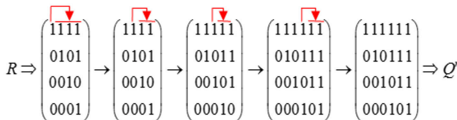
FIGURE 3 | Example of constructing the Q_r matrix based on the Augment Algorithm.
