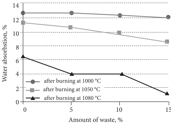
Fig. 5. Influence of the amount of waste on water absorption
