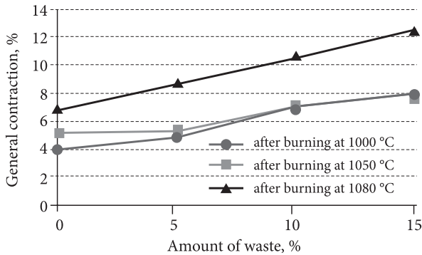
Fig. 4. General contraction of the samples
