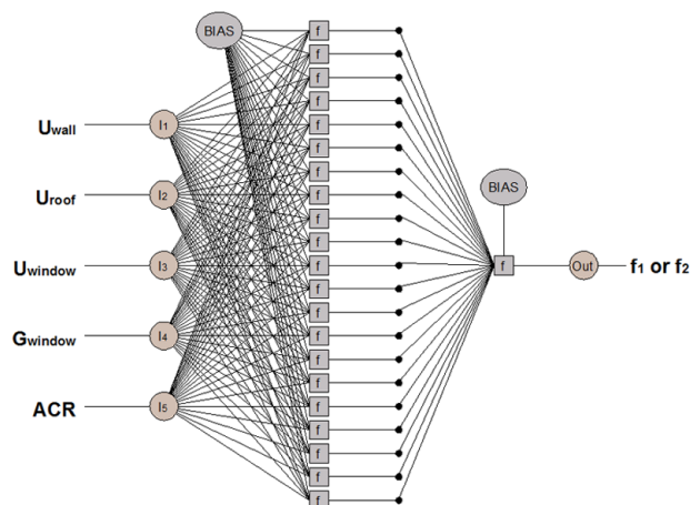
Fig. 1. Artificial neural networks architecture
