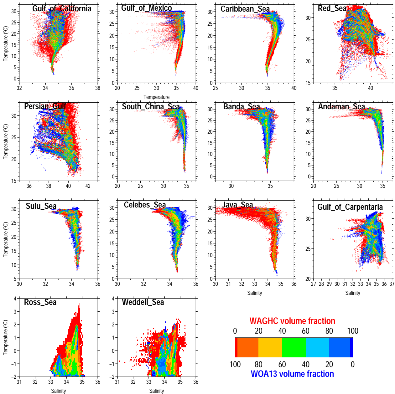
Figure 13. T – S histograms for selected areas of the world ocean (see Fig. 12) for WAGHC and WOA13 gridded climatologies. Bin size is 0.1\text{ }^{\circ}\text{C} \times 0.05\text{ psu} . Colors represent the volume fraction of each climatology. Please note that the above figure contains disputed territories.
