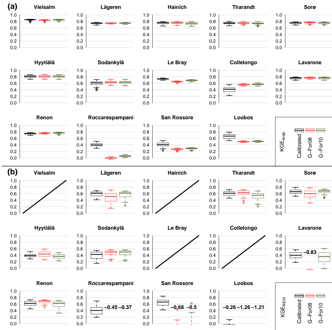
Figure 8. KGE scores obtained during the validation, for total evaporation E_{\text{tot}} (a) and relative extractable soil moisture REW (b). The boxes in each plot correspond to the three sets of validation runs listed in Table 3 (parameter sets derived from calibration, and their two variants with S_r replaced with the value from the G-For08 and G-For10 models). The center of the boxes represents the median of KGE scores, and the lower and upper bounds of the boxes show the first and third quartiles, respectively. The whiskers extend to the furthest values within 1.5 times the interquartile range (IQR) from the box bounds. Where the majority of KGE scores are below zero, the median is printed on the plot. No validation runs were done for Wetzstein, due to the short data record. Also, no soil moisture time series were available for validation at the four sites for which the graphs are crossed out on (b).
