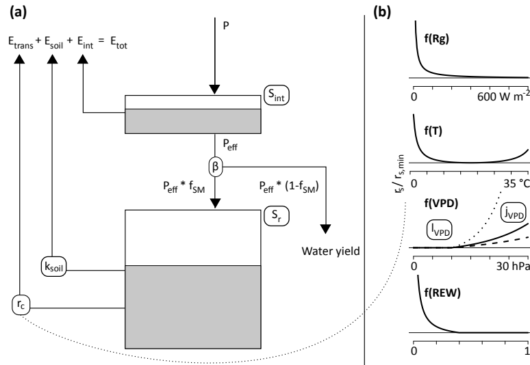
Figure B1. (a) Schematic representation of the water fluxes in the FORHYTM local water balance model. Incoming precipitation P first fills a canopy interception reservoir of size S_{\text{int}} , from which water evaporates back to the atmosphere. Precipitation reaching the ground, P_{\text{eff}} , is split between the rooting zone storage and runoff/groundwater recharge as a function of the parameter \beta and the current filling status of the rooting zone storage. This storage is depleted by soil evaporation and overstory transpiration. Soil evaporation is reduced from its potential value as a function of time since the last rainfall and the parameter k_{\text{soil}} . Transpiration is controlled by the canopy resistance r_c , i.e., stomatal resistance divided by LAI. (b) Relative increase in stomatal resistance as a function of radiation, air temperature, VPD and REW. When all functions are equal to one (optimal conditions), stomatal resistance is equal to r_{s,\min} .
