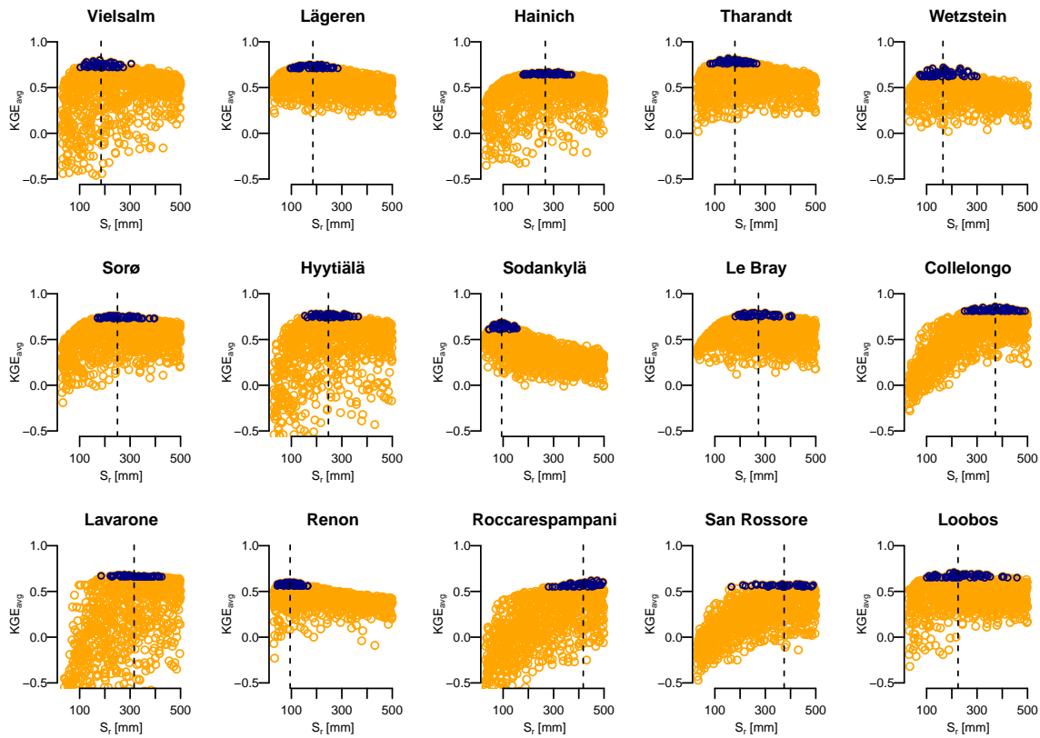
Figure 3. Relationship of the KGE_{avg} obtained during calibration and the parameter values of S_r . The dark blue points have a KGE_{avg} greater than or equal to the 95th percentile at this site, and the line shows the median of these values (i.e., the value reported in Table 5). Although KGE_{avg} scores lower than -0.5 occur at some sites, the y-axis has been truncated in these graphs for clarity. At most sites, the KGE_{avg} scores decrease faster with S_r smaller than the optimal range than they do with larger S_r .
