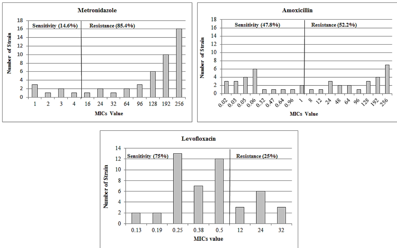
Fig.2: Distribution of Metronidazole, Amoxicillin and Levofloxacin MIC value.
