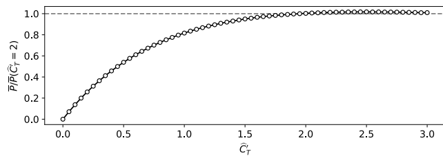
Figure 6. Normalized power extraction as a function of steady thrust coefficient \hat{C}_T' for wind turbines subject to the same free-stream turbulent inflow as in case C3t5. Every dot corresponds to one LES.
