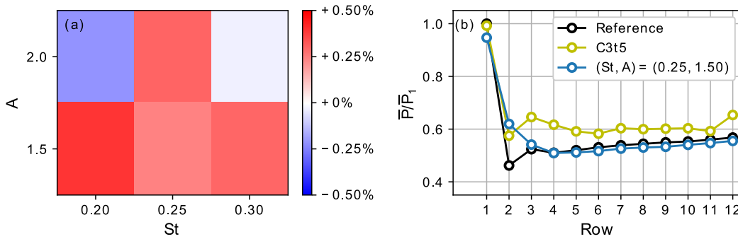
Figure 19. Power extraction of full-scale sinusoidal thrust case ( S = 6D , z_0 = 10^{-1} m). (a) Relative gain in mean wind-farm power extraction over reference case as a function of sine amplitude A and frequency St . (b) Row-averaged mean power extraction for the sinusoidal case with parameters from previous sections, the optimal control case C3t5 from MM17, and the reference case normalized by first-row reference power.
