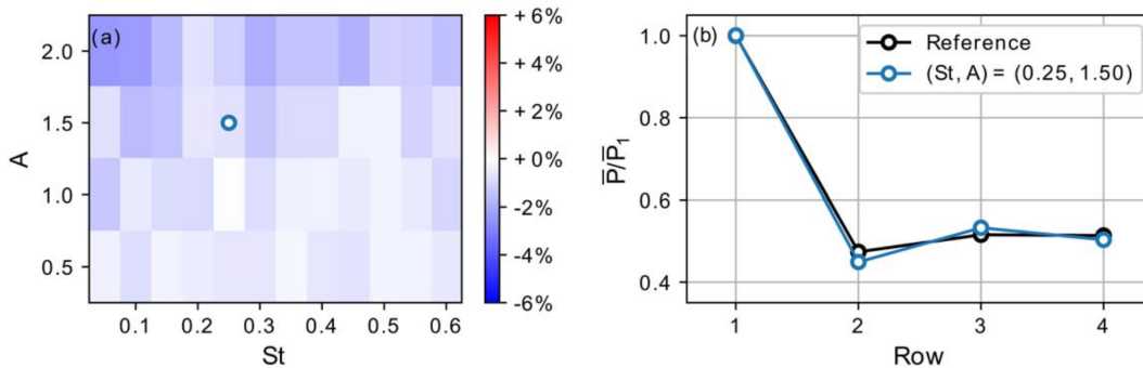
Figure 16. Power extraction of second-row sinusoidal thrust case. (a) Relative gain in mean wind-farm power extraction over reference case as a function of sine amplitude A and frequency St . (b) Row-averaged mean power extraction for the sinusoidal case with the optimal parameters as for row 1 sinusoidal thrust and the reference case normalized by first-row reference power.
