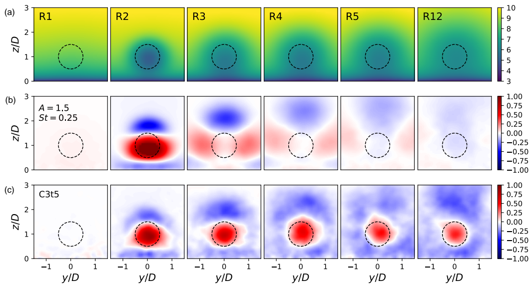
Figure 20. Cross section of time-averaged axial velocity \tilde{U}_x at rotor locations in rows 1, 2, 3, 4, 5, and 12. (a) Reference case. (b) Difference between best sinusoidal perturbation case (with A = 1.5 , St = 0.25 ) and reference case. (c) Difference between optimal control case C3t5 and reference case. Coloring is in units of \text{m s}^{-1} .
