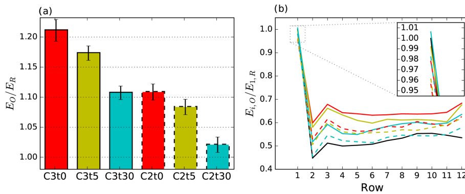
Figure 3. Energy extraction E_O of optimally controlled wind-farm cases from MM17 normalized by a greedy reference case E_R . (a) Total energy extraction. Error bars indicate confidence intervals of \pm 2 standard deviations. (b) Energy extraction by row normalized by first-row reference power. C3t0, red line; C3t5, yellow line; C3t30, blue line; C2t0, red dashed line; C2t5, yellow dashed line; C2t30, blue dashed line. Figure originally published in Munters and Meyers (2017) under a CC-BY 4.0 license.
