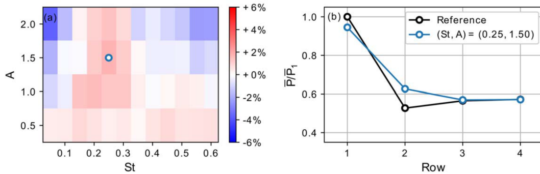
Figure 18. Power extraction of sinusoidal thrust case with increased wall roughness z_0 = 1 m. (a) Relative gain in mean wind-farm power extraction over reference case as a function of sine amplitude A and frequency St . (b) Row-averaged mean power extraction for the best sinusoidal case and the reference case normalized by first-row reference power.
