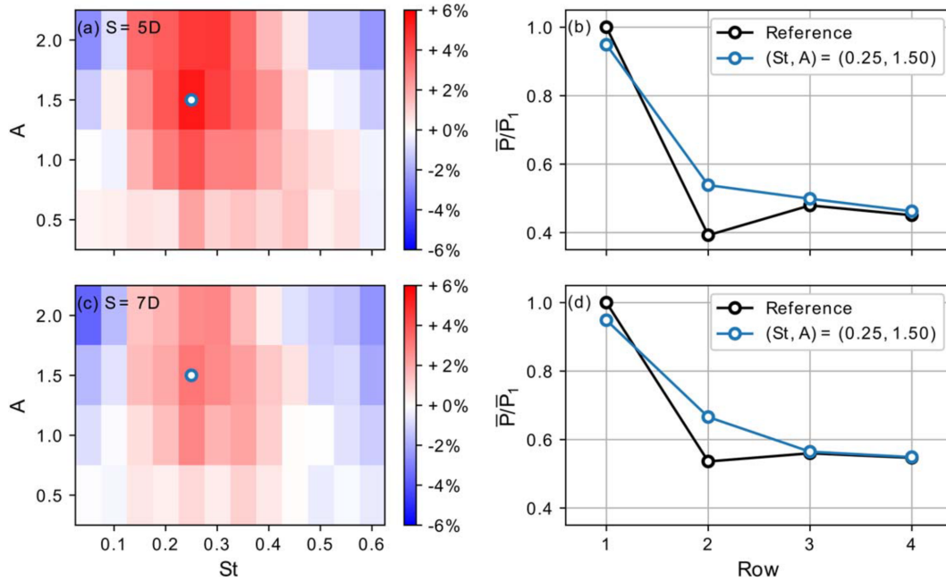
Figure 17. Power extraction of sinusoidal thrust cases with varying streamwise spacing. (a, b) Decreased spacing at S = 5D . (c, d) Increased spacing at S = 7D . (a, c) Relative gain in mean wind-farm power extraction over reference case as a function of sine amplitude A and frequency St . (b, d) Row-averaged mean power extraction for the best sinusoidal case and the reference case normalized by first-row reference power.
