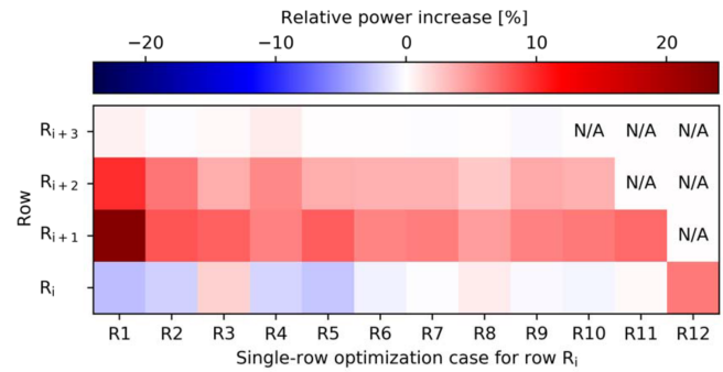
Figure 10. Relative power increase matrix for downstream rows in the single-row optimization case for row R_i , indicated in the horizontal axis. N/A indicates nonexisting downstream rows. Finite-horizon effects are eliminated by only reporting a power increase up to t = T_A for the active row R_i .
