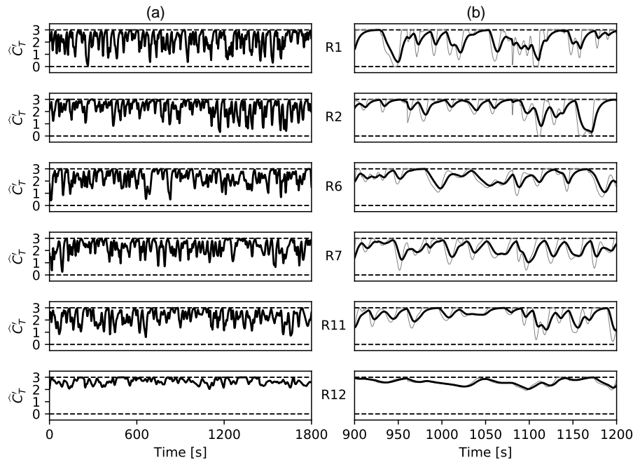
Figure 5. Time evolution of the thrust coefficient \hat{C}_T' for a selection of optimally controlled turbines in case C3t5. (a) Total time horizon. (b) Zoomed view including set point C_T' in gray.
