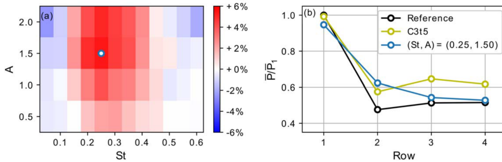
Figure 14. Power extraction of baseline sinusoidal thrust case ( S = 6D , z_0 = 10^{-1} m). (a) Relative gain in mean wind-farm power extraction over reference case as a function of sine amplitude A and frequency St . (b) Row-averaged mean power extraction for the best sinusoidal case, the optimal control case C3t5 from MM17, and the reference case normalized by first-row reference power.
