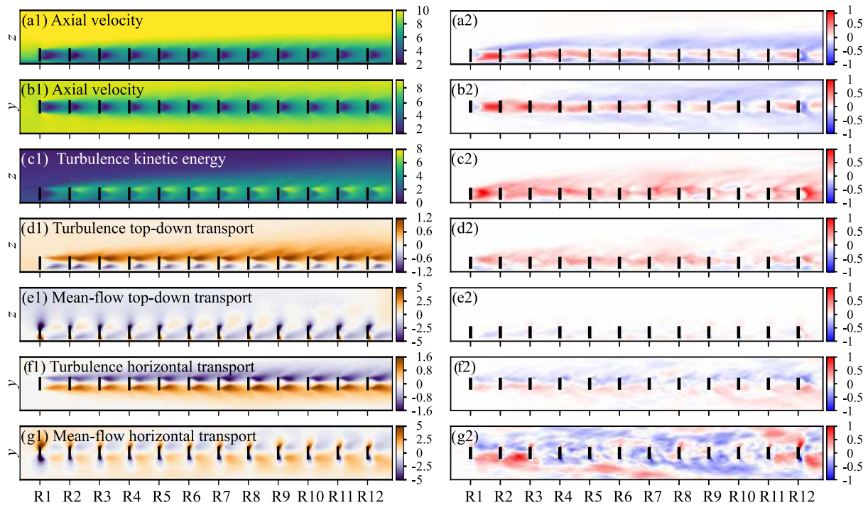
Figure 4. Time-averaged flow field quantities of simulation results from MM17. Left: time averages of reference simulations with C'_T = 2 for all turbines. Right: difference \Delta between reference and optimal control (C3t5) simulation, defined as \Delta = X_{C3t5} - X_{REF} for any variable X . (a) Axial velocity U_x (plan view at hub height). (b) Axial velocity U_x (side view through turbine column). (c) Turbulence kinetic energy k = (1/2)(\overline{u'_x u'_x} + \overline{u'_y u'_y} + \overline{u'_z u'_z}) (side view). (d) Turbulence top-down transport -\overline{u'_x u'_z} . (e) Mean flow top-down transport -\overline{U_x U_z} (side view). (f) Turbulence horizontal transport \overline{u'_x u'_y} (plan view). (g) Mean flow horizontal transport \overline{U_x U_y} (plan view). Black lines indicate wind turbine locations. Simulation results are averaged over the six different wind turbine columns.
