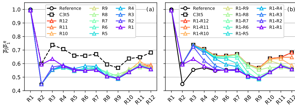
Figure 8. Normalized row-averaged power extraction for the reference case, optimal control case C3t5, and subset control cases up to optimization window 3. (a) Subset control cases with optimal controls applied only in one specific row. (b) Subset control cases with optimal controls applied for all rows up to specific row.
