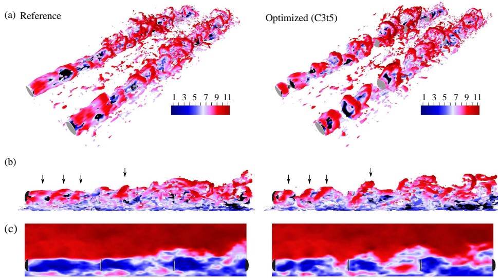
Figure 12. Instantaneous snapshots at t = 300 s of a portion of the wind-farm flow field for the reference (left) and optimized (right) case. (a, b) Isosurface of vorticity magnitude colored by streamwise velocity \tilde{u}_x . Deep-wake regions (with \tilde{u}_x < 4.5 \text{ m s}^{-1} ) are rendered in black. Black arrows indicate the naturally occurring unstable bulges in the reference case and the accompanying vortex rings in the optimized case. (c) Contours of streamwise velocity \tilde{u}_x . Coloring is in units of \text{m s}^{-1} . Wind turbines are represented as gray disks.
