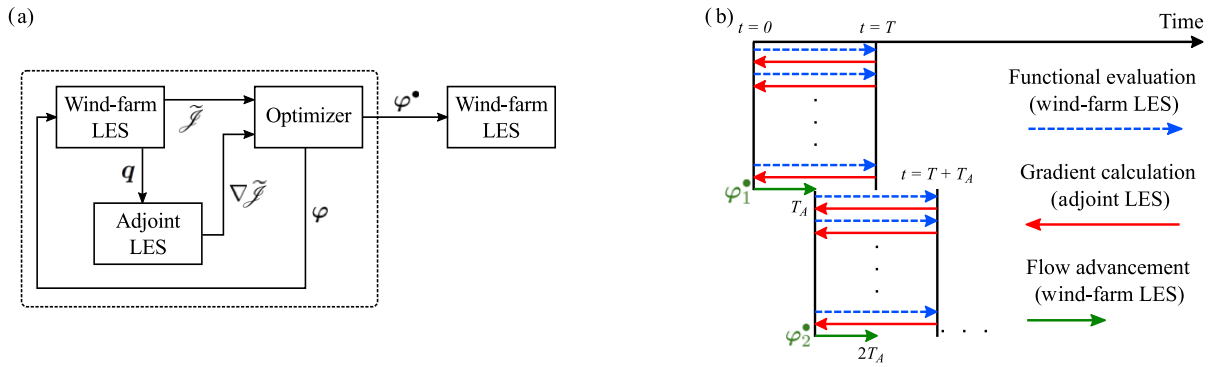
Figure 1. Schematic overview of wind-farm optimal control methodology from MM17. (a) Control block diagram with adjoint gradient-based optimization and LES flow models illustrating data flow of (optimal) controls \varphi^* , system state q , cost functional \mathcal{J} , and its gradient \nabla \mathcal{J} . (b) Receding-horizon framework subdividing time into discrete flow advancement windows of length T_A with prediction horizon T . Each arrow represents a forward or adjoint LES. Every window consists of an optimization stage (blue and red lines) followed by a flow advancement stage with optimal controls \varphi^* (green lines).
