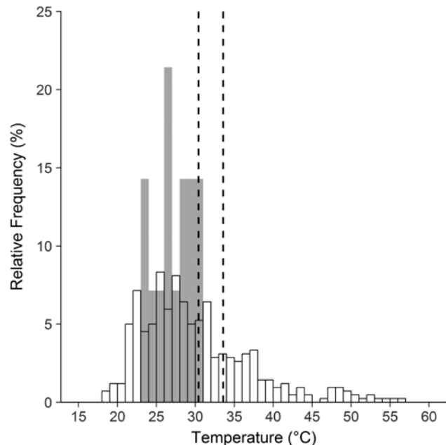
Fig. 2. Relative frequency of field body temperatures ( T_b , grey shade), operative temperatures ( T_e , solid line) and set-point range ( T_{set} , dotted lines) for the Ocellated Skink.
