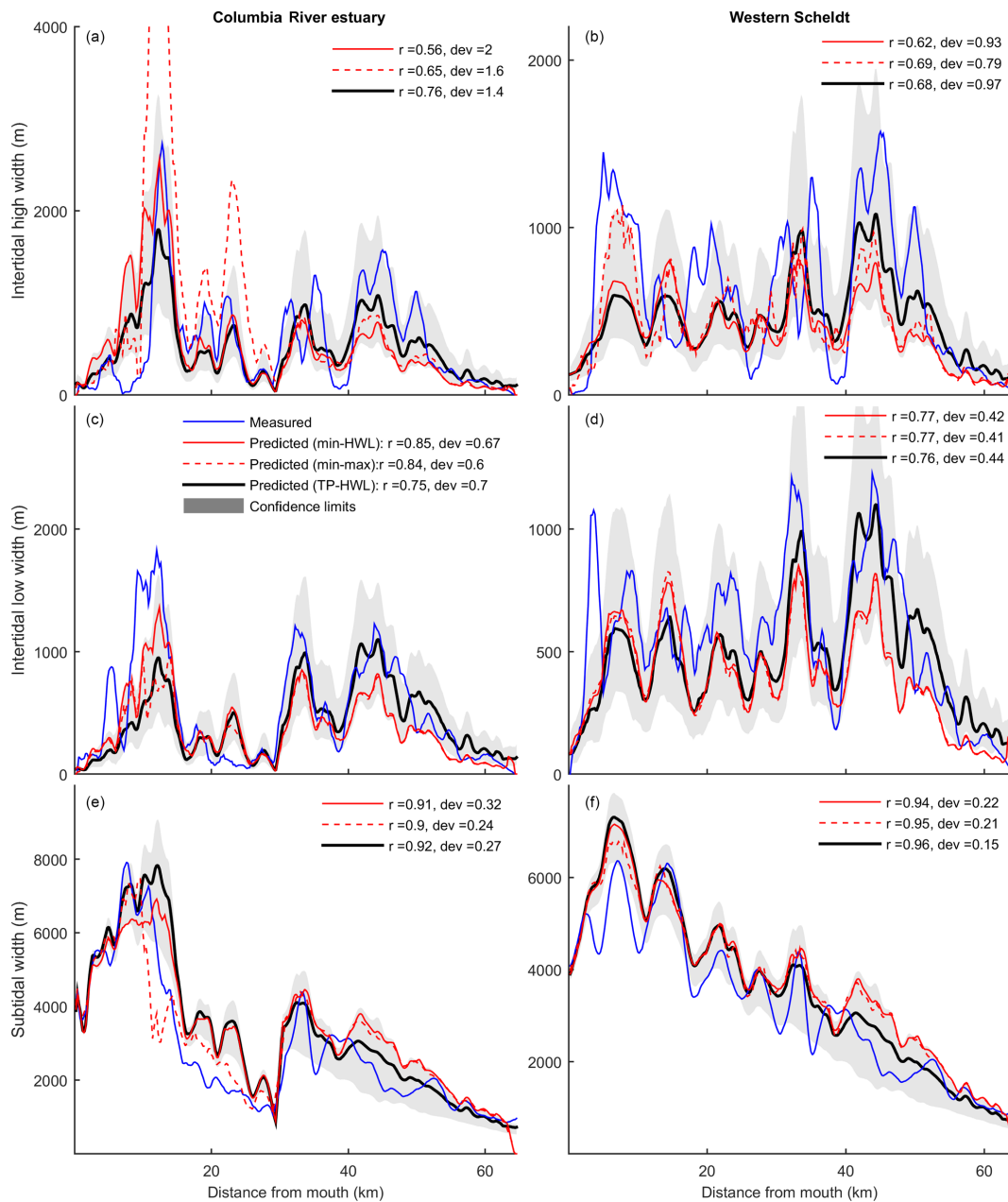
Figure 10. Comparison of measured and predicted values of intertidal high, intertidal low and subtidal width for the Columbia River Estuary (a, c, e) and the Western Scheldt (b, d, f). Predicted nondimensional hypsometry was dimensionalised for each cross section using three methods (explained in Methods) and uncertainty margins are given for one of the predictions (solid black line). In the legend, r indicates the Pearson product-moment correlation coefficient and “dev” the average factor of deviation between the predicted (TP-HWL) and measured lines.
