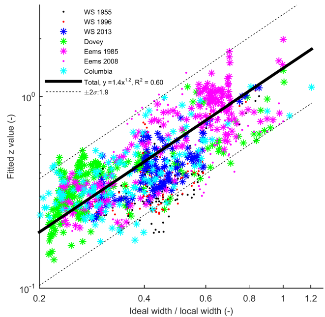
Figure 8. Fitted z values of filtered data increase with the fraction of ideal width and local width, which indicates that hypsometric shapes become progressively more concave when the local width approaches the ideal width and become more convex when the local width becomes larger than the ideal width (i.e. the excess width increases). The data shown as asterisks are used for the regression. Confidence limits are plotted at 2 standard deviations above and below the regression and their multiplication factor compared to the trend is given in the legend.
