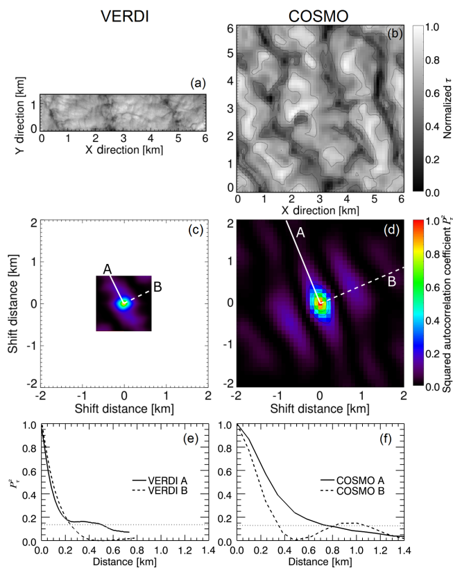
Figure 4. (a–b) Horizontal fields of normalized \tau_{\text{meas}} (VERDI) and \tau_{\text{sim}} (COSMO) for the case on 15 May 2012. (c–d) Two-dimensional autocorrelation coefficients P_{\tau, \text{meas}}^2 and P_{\tau, \text{sim}}^2 , calculated for fields of \tau displayed in panels (a) and (b). (e–f) One-dimensional autocorrelation coefficients along (straight white line marked in panels c and d) and across (dashed white line marked in panels c and d) predominant directional structure. The grey dotted line illustrates the threshold for the estimation of \xi_{\tau}^{\updownarrow} and \xi_{\tau}^{\leftrightarrow} .
