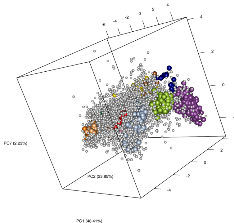
Figure 9. Using the plot3D function to visualise the hl dataset along PCs 1, 2 and 7.
