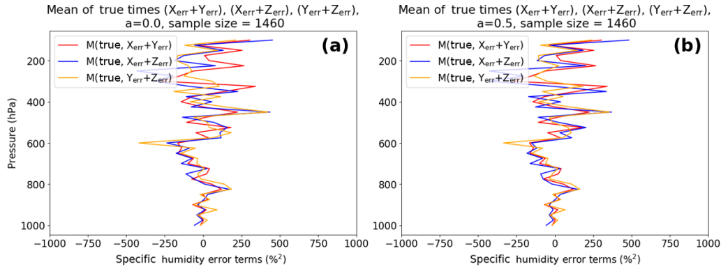
Figure 5. Terms involving products of true and (X_{\text{err}} + Z_{\text{err}}) , (X_{\text{err}} + Y_{\text{err}}) and (Y_{\text{err}} + Z_{\text{err}}) for (a) a = 0 and (b) a = 0.5 . Note that the magnitudes of true and (X_{\text{err}} + Y_{\text{err}}) and true and (Y_{\text{err}} + Z_{\text{err}}) do not depend on the correlation between X_{\text{err}} and Z_{\text{err}} . All error terms are normalized.
