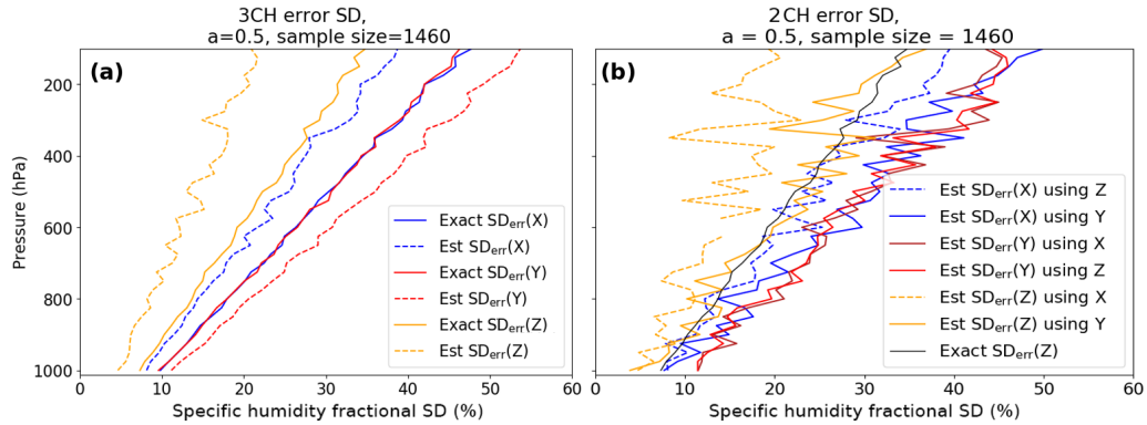
Figure 8. Estimated and exact normalized error standard deviations for 3CH method (a) and 2CH method (b) for a correlation of Z and X errors of 0.45 ( a = 0.5 ). (a) Exact SD err (X) errors for X, Y and Z are given by blue, red and orange solid lines, respectively. Estimated error SD error is given by dashed lines of same color. (b) Exact error SD of Z is given by solid black line. Estimated error SD of X using Z and Y is given by blue lines, estimated error SD of Y using X and Z is given by red lines, and estimated error SD of Z using X and Y is given by orange lines. For all colored lines, error terms are neglected. Solid lines indicate estimates from combinations of data sets with uncorrelated errors, dashed lines indicate estimates from combinations of data sets with correlated errors and hence larger error terms.
