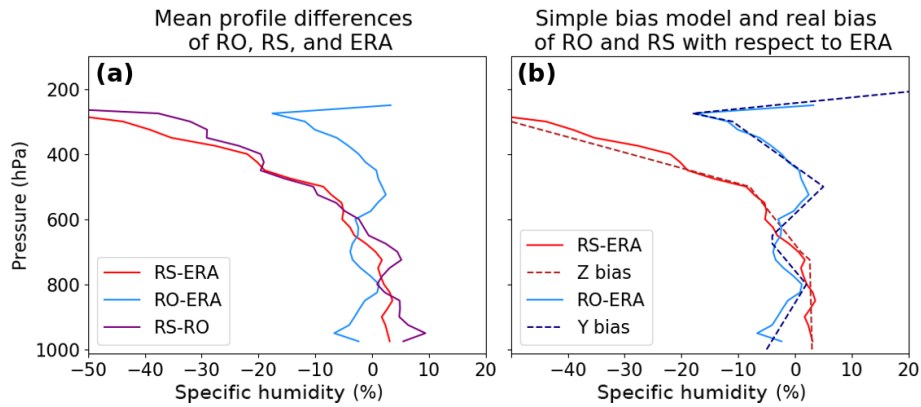
Figure 13. (a) Annual mean normalized profiles of RS–ERA, RO–ERA and RS–RO. (b) Same for RS–ERA and RO–ERA only (solid lines), and their respective empirical bias profiles (dashed lines) based on the mean profiles.
