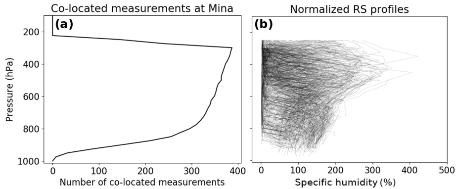
Figure 11. (a) Number of co-located measurements (data pairs) per pressure level for RO, RS and ERA. (b) Normalized q values for radiosondes (RS) at Mina, 2007. The normalized q values are computed as 100 \cdot q/\bar{q} , where \bar{q} is the annual mean value of q for 2007. Profiles cut off at 250 hPa because RS data are not reported at higher levels. At the bottom, co-located profiles thin out since RO penetration depth varies and only very few profiles are available at the lowest levels.
