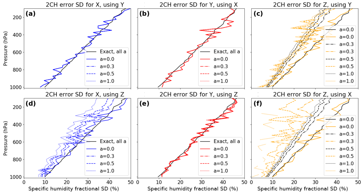
Figure 7. Two 2CH results each for the normalized error SD for X (a, d), Y (b, e) and Z (c, f), depending on the second data set. Profiles corresponding to several values of correlation parameter a are included. The solid black profile is the exact error SD profile for X and Y for all values of a , and for Z when a = 0 .
