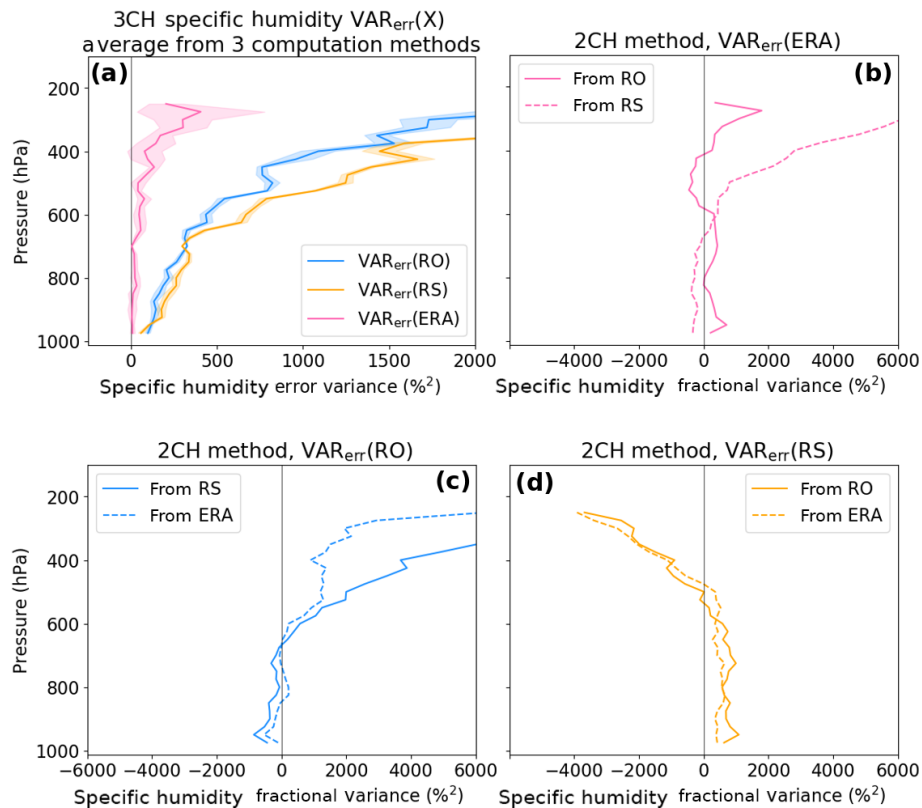
Figure 12. Estimated error variances for specific humidity: (a) results from the 3CH method for ERA (purple), RO (blue) and RS (orange). Other three panels: 2CH method estimates for ERA (b), RO (c) and RS (d).
