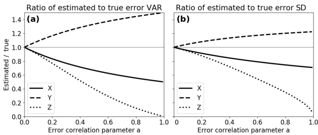
Figure 4. Ratio of estimated (a) error variances to true variances and (b) estimated SD to true SD for the 3CH method for values of error correlation parameter a ranging from 0 to 1.0.
