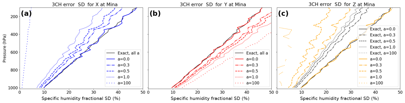
Figure 3. (a) Estimated standard deviation of X_{err} for values of a = 0, 0.3, 0.5, 1.0 and 100 computed from Eqs. (3a)–(5a). Exact SD computed from data set X (solid black profile). (b) Same as (a) except for estimated SD of Y_{err} . (c) Same as (a) except for estimated SD of Z_{err} . Note that for different values of a , the exact SD of X_{err} and Y_{err} are always the same. The exact SD of Z_{err} decreases as a increases for 0 < a < 1.0 . For a > 1.0 , the exact SD of Z_{err} increases as a increases, becoming equal to the SD of X_{err} for a = \infty due to the way our error model is defined (see also Table 1). For a = 100 the correlation between X and Z errors is 0.99995 (Table 1; black dotted line for a = 100 almost identical to black solid line for a = 0 ).
