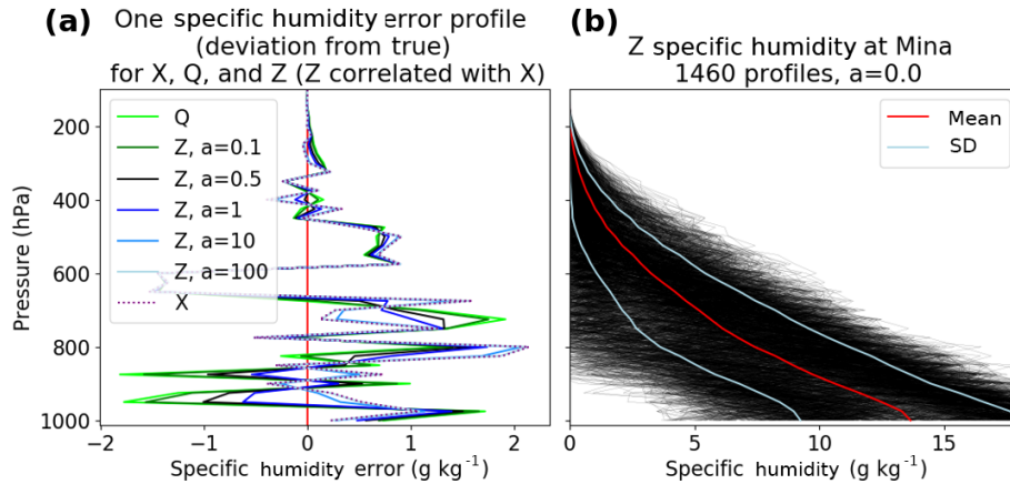
Figure 1. (a) One set of error profiles with the unnormalized X_{err} (dotted line), Q_{err} (solid lime green line) and Z_{err} (various solid lines for different values of correlation parameter a ). Q_{err} is uncorrelated with X_{err} . For a = 0 , Z_{err} = Q_{err} and Z_{err} and X_{err} are uncorrelated. As a increases, Z_{err} is increasingly correlated with X_{err} and looks less like Q_{err} and more like X_{err} . For very large a ( a = 100 ), Z_{err} (light blue solid line) is almost equal to X_{err} (dotted line). (b) 1460 profiles of the unnormalized data set Z with zero correlation with X ( a = 0 ).
