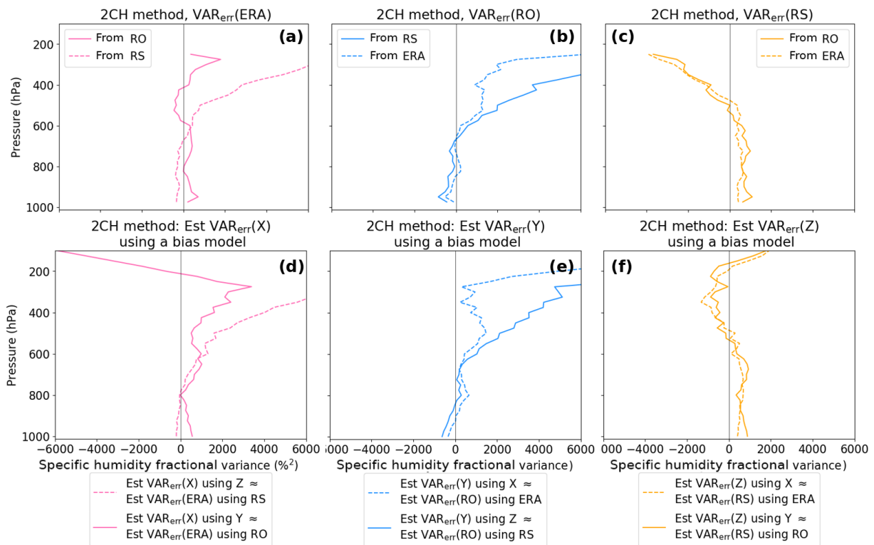
Figure 14. 2CH method error variances for ERA, RO and RS (a–c) and for simulated data using the specified empirical bias profiles (d–f). Correlation between X and Z errors is zero for this experiment.
