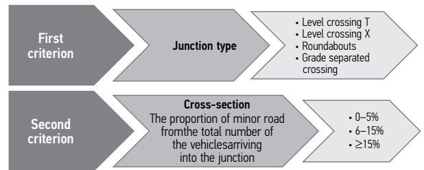
Fig. 2. The process of dividing the junctions into junction groups and subgroups
