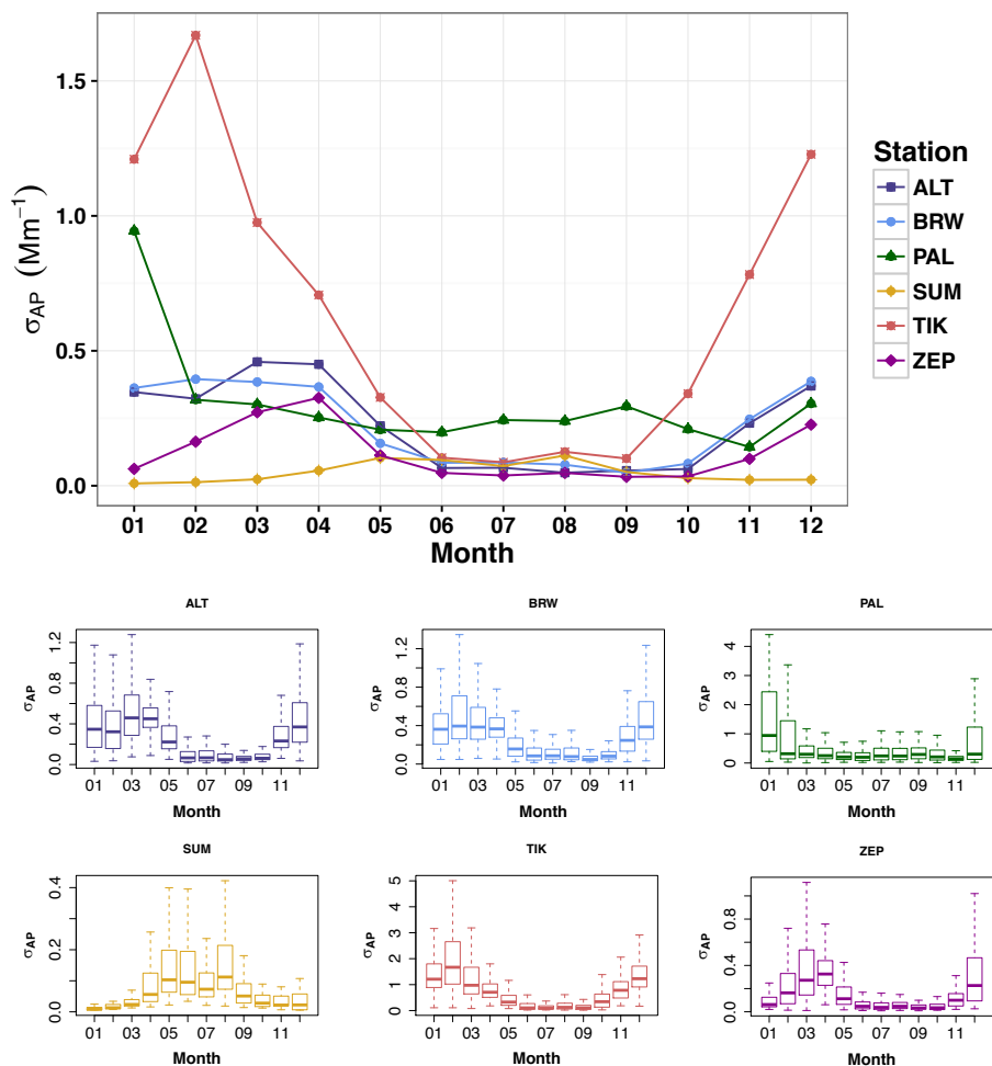
Figure 4. Seasonality of aerosol light absorption coefficient ( \sigma_{ap} ) at 550 nm at all sites. Large plot shows monthly medians of absorption per megameter ( \text{Mm}^{-1} ) at each station; subplots below show boxplots of hourly average absorption at individual sites, with horizontal line at the median, edges of the box at 25th and 75th percentiles, and whiskers at 5th and 95th percentiles. Note that y axes are different on each plot. Size cuts for the Aethalometer absorption measurements are as follows: 10\ \mu\text{m} (ALT); 2.5\ \mu\text{m} (SUM); 10\ \mu\text{m} (TIK); and no size cut at BRW, PAL, and ZEP.
