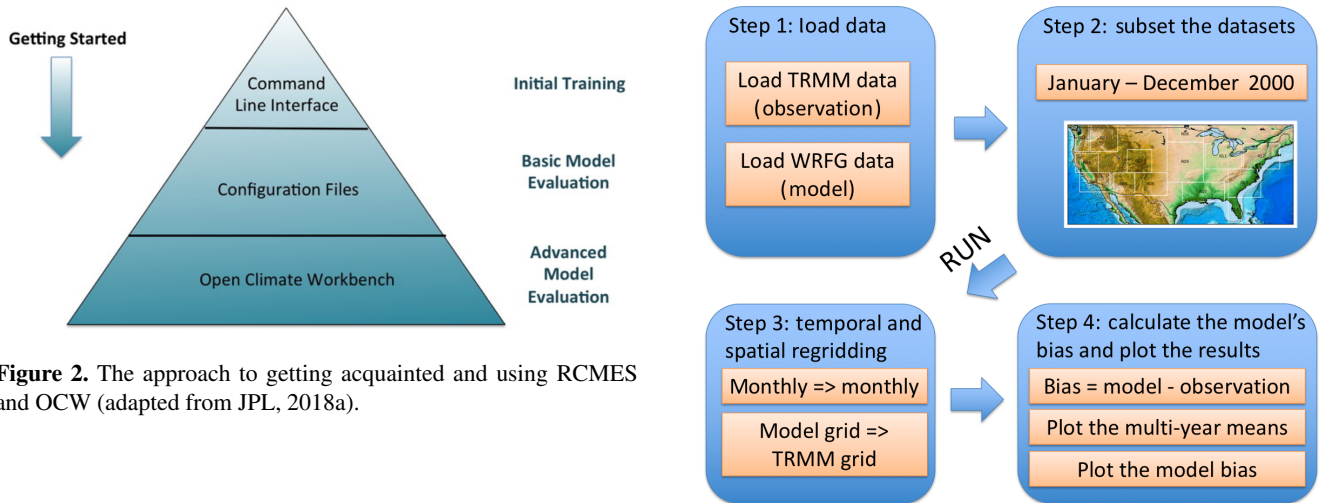
Figure 3. The four steps of model evaluation included as a CLI example of RCMES.
