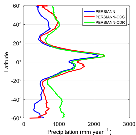
Figure 7. Mean annual zonal precipitation ( \text{mm yr}^{-1} ) for PERSIANN, PERSIANN-CCS, and PERSIANN-CDR.
