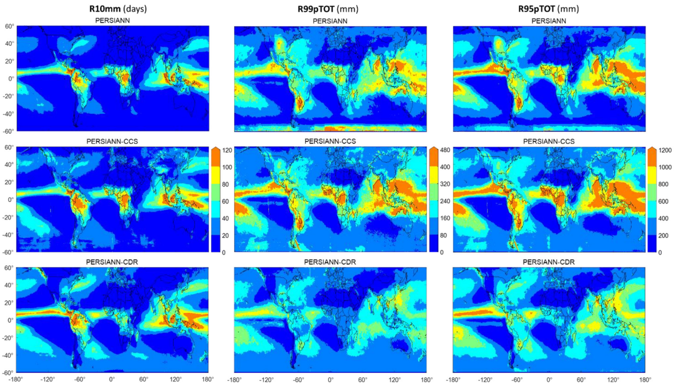
Figure 11. Extreme precipitation indices (R10mm, R99pTOT, and R95pTOT) for PERSIANN, PERSIANN-CCS, and PERSIANN-CDR over the globe. (See Table 4 for definitions of the indices.)
