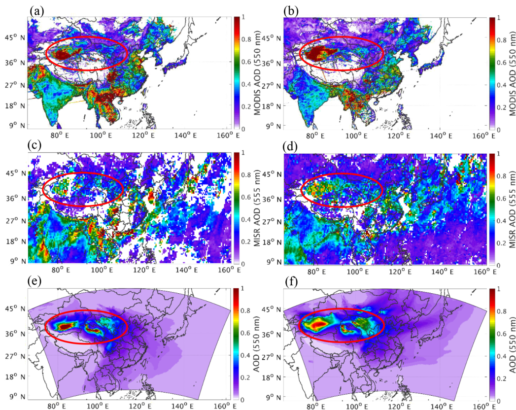
Figure 5. Spatial distributions of monthly mean AOD from MODIS observations (a, b), MISR observations (c, d), and simulation results (e, f) for March (left column) and April (right column) of 2012.
