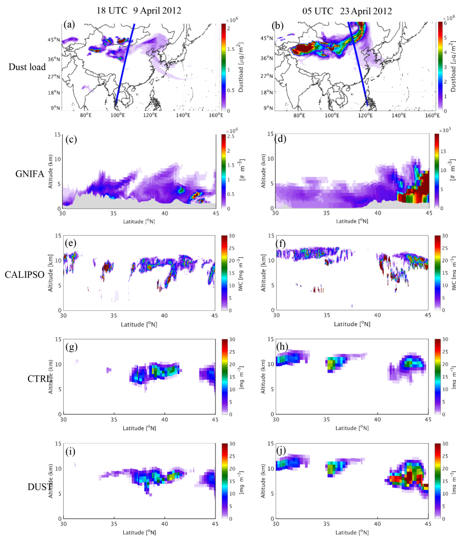
Figure 9. As Fig. 8 but for the cases on 9 April (left column) and 23 April (right column) of 2012.
