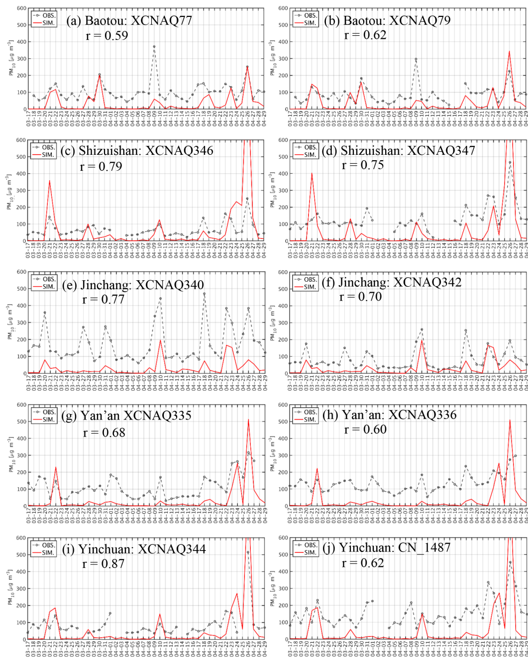
Figure 3. Time series of hourly observed and simulated surface \text{PM}_{10} concentrations at various environmental monitoring stations; r represents the correlation coefficient between simulation results and observations.
