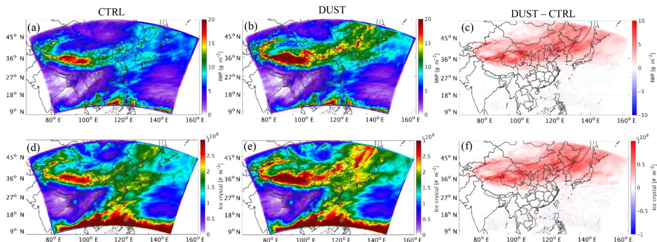
Figure 7. Spatial distributions for the temporal mean simulated cloud ice water path (a–c) and ice crystal number density (d–f) from CTRL (left column), DUST (middle column), and the difference between CTRL and DUST (right column) over East Asia (domain 1) during the simulation period.
