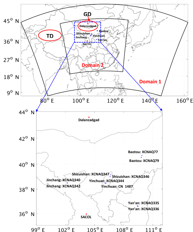
Figure 1. Nested domain set for the simulations. Blue dots represent the 10 monitoring stations used for model validation. TD: the Taklimakan Desert; GD: the Gobi Desert.
