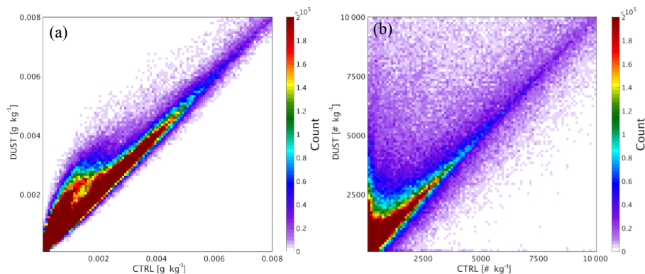
Figure 6. 2-D histogram of simulated cloud ice mixing ratio (a) and cloud ice crystal number concentration (b) from CTRL and DUST. The color scales indicate the number of grid points in specific value bins of ice mixing ratio and ice crystal number concentration.
