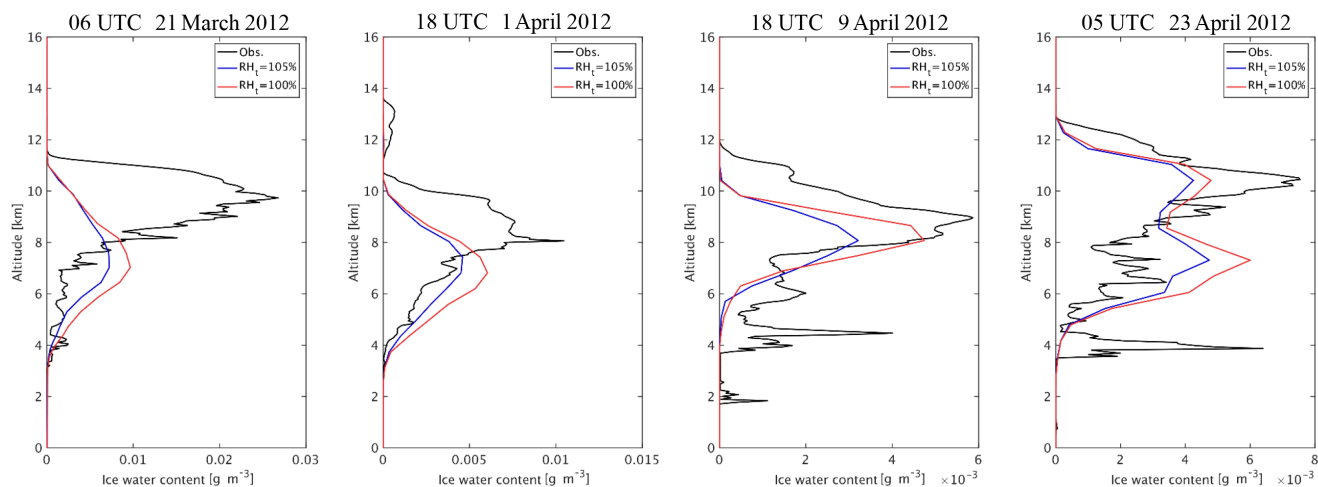
Figure 12. Vertical profiles for the mean observational IWC from CALIPSO and the simulated IWC with threshold RH values of 105 and 100 % for the dust events on 21 March and 1, 9, and 23 April 2012.
