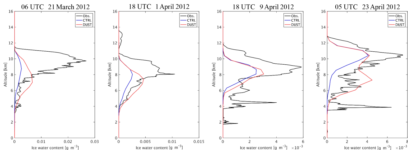
Figure 10. Vertical profiles for the mean observed IWC from CALIPSO and the simulated IWC from CTRL and DUST for dust events on 21 March and 1, 9, and 23 April 2012.
