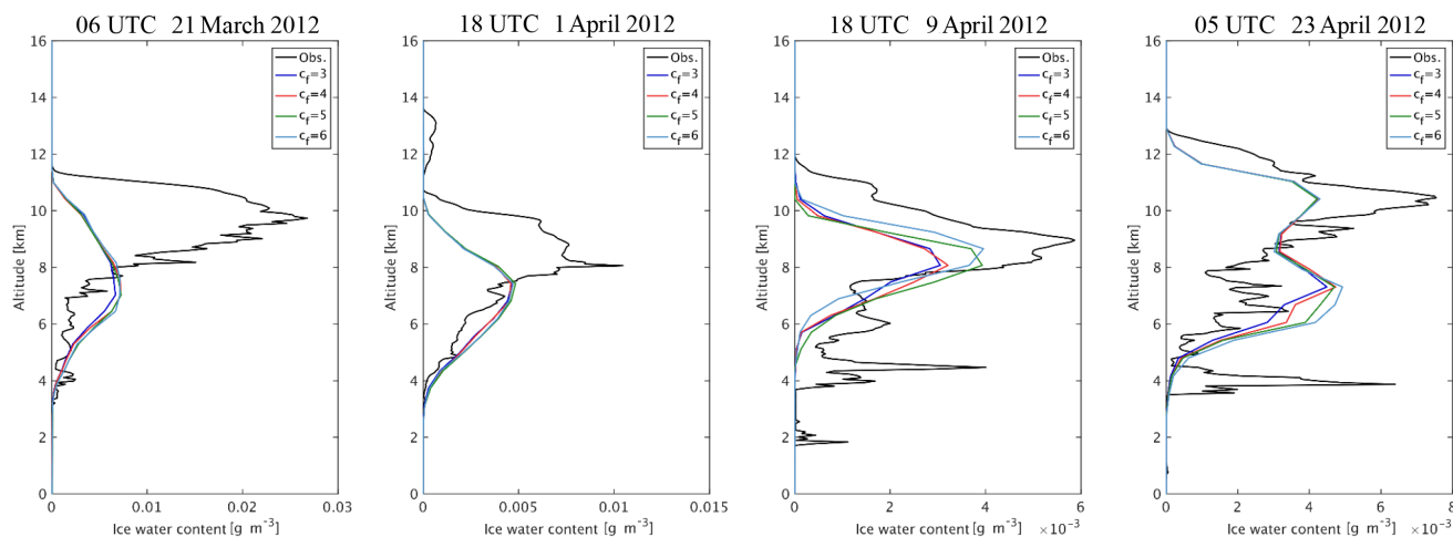
Figure 11. Vertical profiles for the mean observed IWC from CALIPSO and the simulated IWC with various c_f for the dust events on 21 March and 1, 9, and 23 April 2012.
