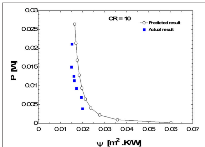
FIGURE 8 | Power output P vs. system parameter \psi at CR = 10.
