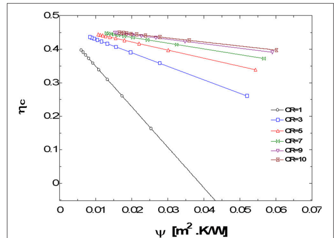
FIGURE 5 | Collector efficiency \eta_c vs. system parameter \psi at different concentration ratios.
