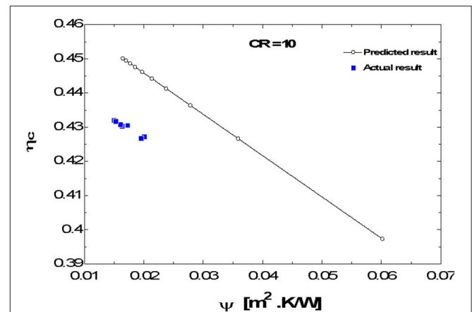
FIGURE 6 | Collector efficiency \eta_c vs. system parameter \psi at CR = 10.
