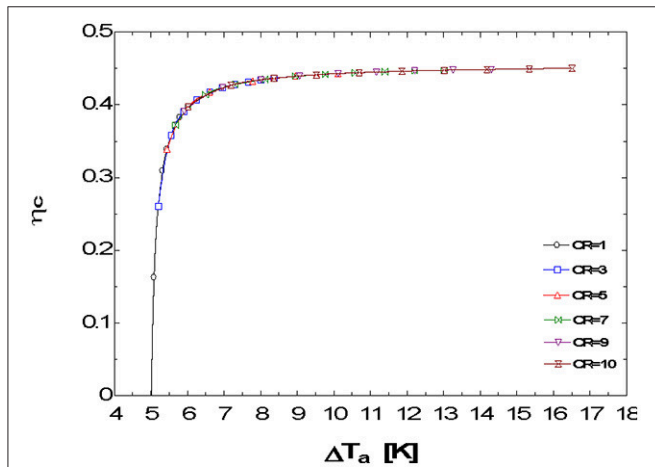
FIGURE 3 | Collector efficiency \eta_c vs. temperature difference \Delta T_a at different concentration ratios.
