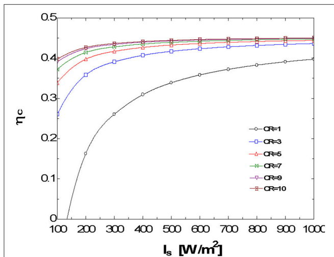
FIGURE 4 | Collector efficiency \eta_c vs. insolation I_s at different concentration ratios.
