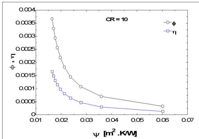
FIGURE 7 | Conversion efficiency \phi , overall efficiency \eta vs. system parameter \psi at CR = 10.
