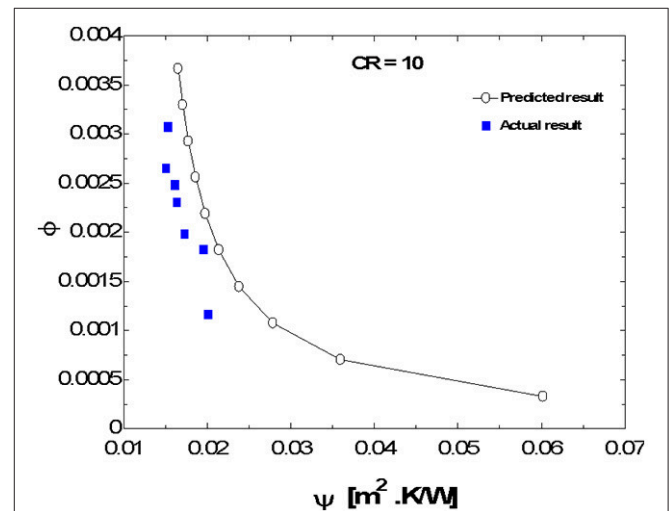
FIGURE 9 | Conversion efficiency, \phi , vs. system parameter \psi at CR = 10.
