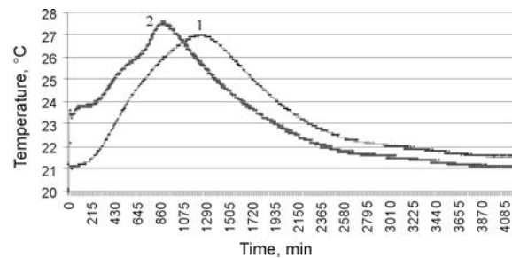
Fig. 4. The temperatures of the exothermic effect of the expanded-clay lightweight concrete during the hardening Note: 1 – expanded-clay lightweight concrete without the waste material, when water/concrete ratio is 0.52; 2 – expanded-clay lightweight concrete with 15% of waste material, water/cement ratio is 0.61
