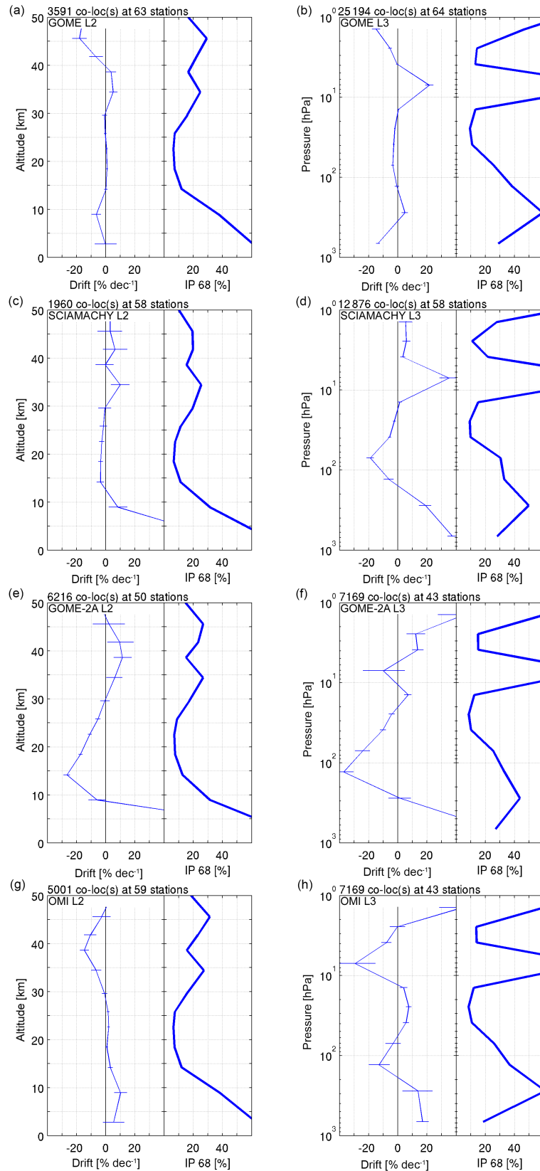
Figure 12. Relative decadal drift and 68 % interpercentile spreads for comparisons of L2 (a, c, e, g) and L3 (b, d, f, h) GOME, SCIAMACHY, GOME-2A, and OMI data (top to bottom panels) with ground-based reference measurements. Two sigma error bars, resulting from a bootstrapping with 1000 samples, are added to the drift profiles.
