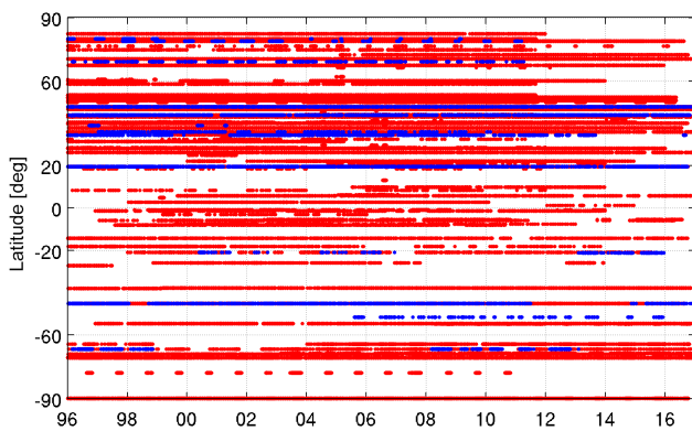
Figure 2. Latitude–time sampling (1996–2016) of the ground-based ozonesonde (red dots) and stratospheric ozone lidar (blue dots) measurements obtained from the NDACC, SHADOZ, and WOUDC reference network databases.
