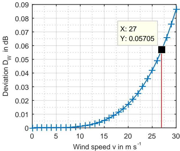
Figure 10. Analytically calculated deviation over the wind velocity. At wind velocity of 27 \text{ m s}^{-1} , WECS are turned off.
