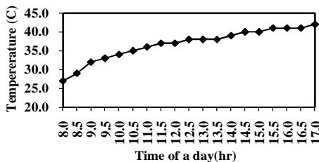
Fig. 4: The temperature of water in the tank vs day time for a variable cloudy day.
