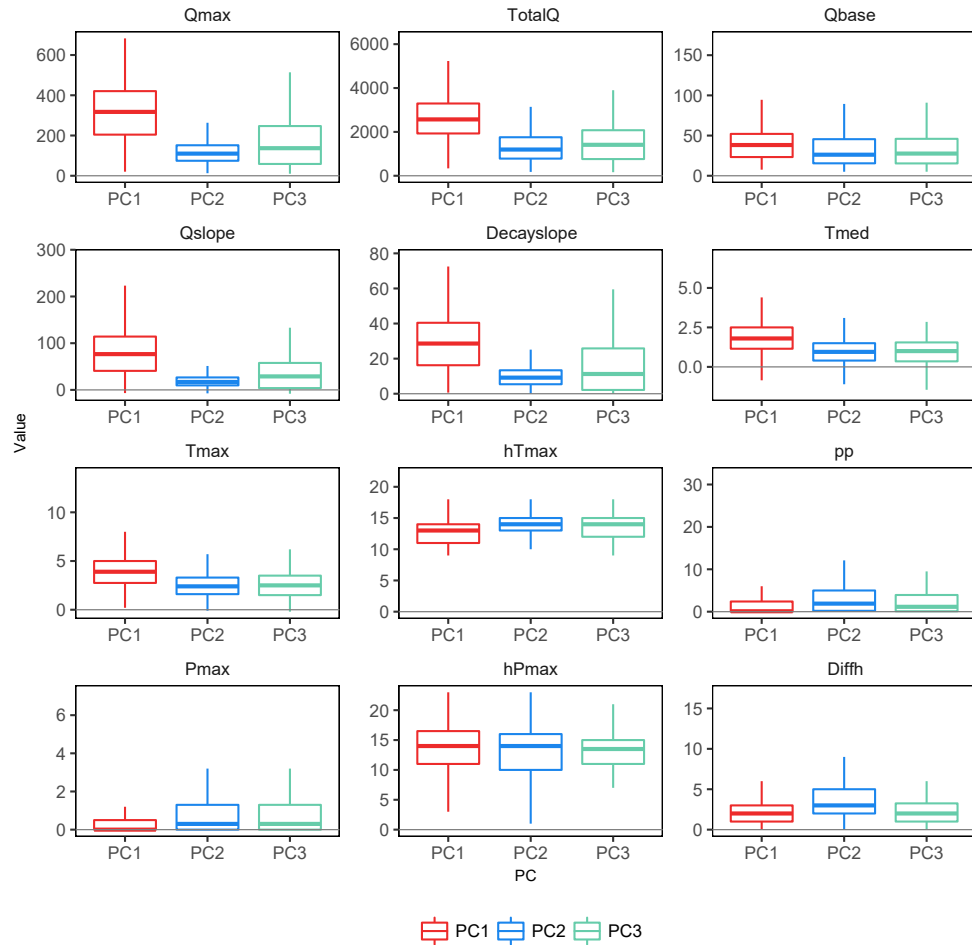
Figure 5. Summary of the frequency distributions (box plots) of the hydrological and meteorological indicators for days grouped within PC1, PC2 and PC3.
