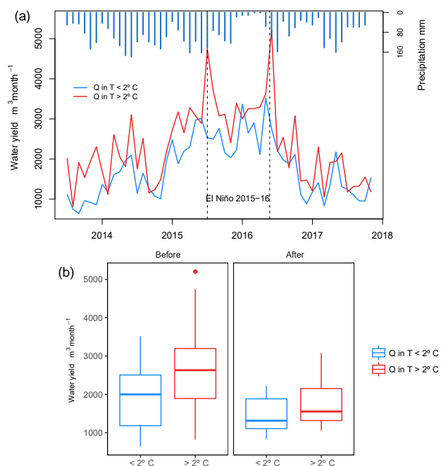
Figure 7. Mean monthly water discharge ( Q ), for days with temperature lower than 2^{\circ}\text{C} (blue) and days with temperature higher than 2^{\circ}\text{C} (red): (a) interannual evolution with indication of El Niño 2015–2016 event (grey shading), breakpoint in water discharge evolution (dashed line) and monthly precipitation (blue bars); (b) comparative box plots for water discharge before and after breakpoint in May 2016.
