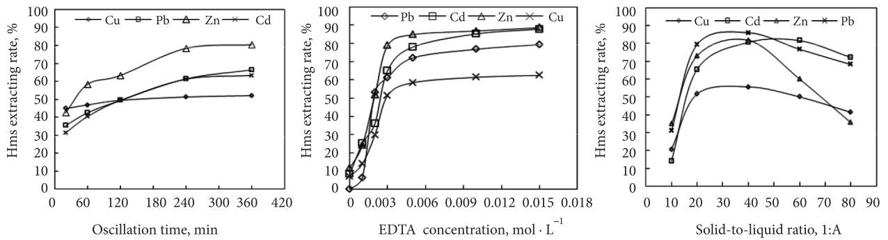
Figure 1. Effect of single process parameter on EDTA enhanced soil washing
