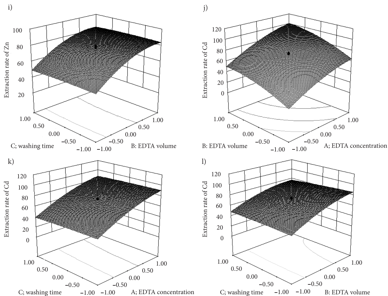
Figure 2. 3D surface showing the interaction effects of variables on extraction rates of various HMs: a) 3D surface of extraction rate of Cu and interaction of AB; b) 3D surface of extraction rate of Cu and interaction of AC; c) 3D surface of extraction rate of Cu and interaction of BC; d) 3D surface of extraction rate of Pb and interaction of AB; e) 3D surface of extraction rate of Pb and interaction of AC; f) 3D surface of extraction rate of Pb and interaction of BC; g) 3D surface of extraction rate of Zn and interaction of AB; h) 3D surface of extraction rate of Zn and interaction of AC; i) 3D surface of extraction rate of Zn and interaction of BC; j) 3D surface of extraction rate of Cd and interaction of AB; k) 3D surface of extraction rate of Cd and interaction of AC; l) 3D surface of extraction rate of Cd and interaction of BC
