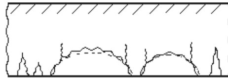
Fig 3. Merge of micro cracks into local cavities
