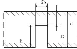
Fig 9. Geometrical model of subsurface defect
