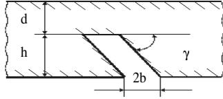
Fig 7. Cross-section of inclined defect
