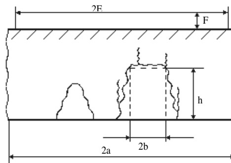
Fig 6. Computational model of subsurface hydrogen corrosion defect
