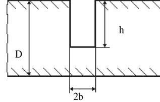
Fig 10. Geometrical model of surface defect
