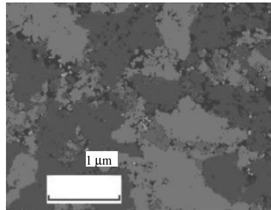
Fig 14. Grains of pressed vanadium carbide VC_{0.875} . Hydrogen corrosion due to steady and pulse irradiation ( \eta = 22 kHz, I = 20 W/sm 2 , \tau = 720 hour). Bright grey area – grains, dark grey – oxide cavities
