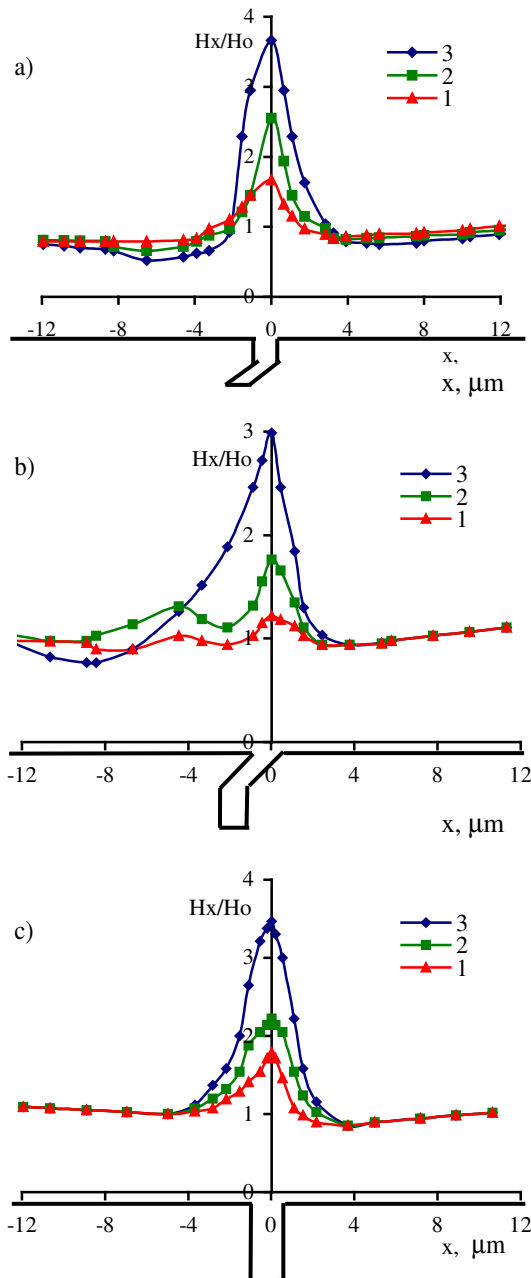
Fig 16. Topography of area with different types of defect ( h = 4 \text{ nm} ; for 1 – 2b = 0.025 \text{ nm} ; 2 – 2b = 0.08 \text{ nm} ; 3 – 2b = 0.2 \text{ nm} ; magnetic intensity on the surface MH: H = 10 \text{ A/cm} )
