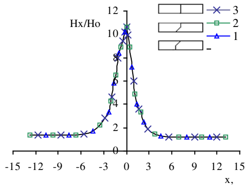
Fig 15. Dependence H_x(x) for three types of defects x, \mu\text{m} ; 2b = 0.2 \text{ nm} in a magnetic field y = 1.0 \text{ nm} , H = 10 \text{ A/sm}
