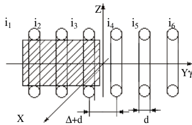
Fig 11. Replacement of three-section coil to six-section coil with infinitely thin conductors
