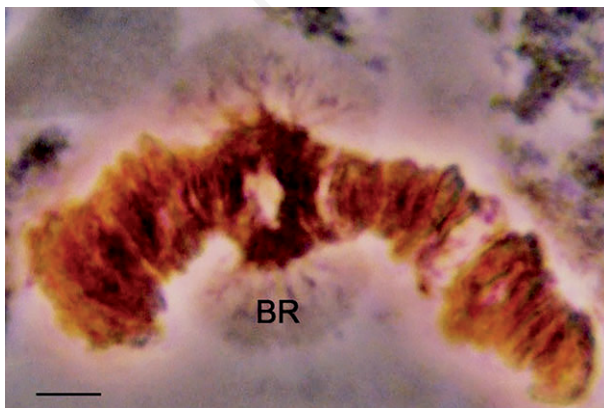
Fig. 1. Representative photomicrograph of chromosome IV from the salivary gland polytene chromosome complements of Chironomus ramosus (Nath and Godbole, 1997) showing a conspicuous Balbiani Ring (BR) at 18C locus. Scale bar: 10 \mu m.
