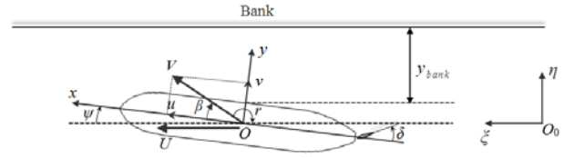
Figure 2. Coordinate systems
