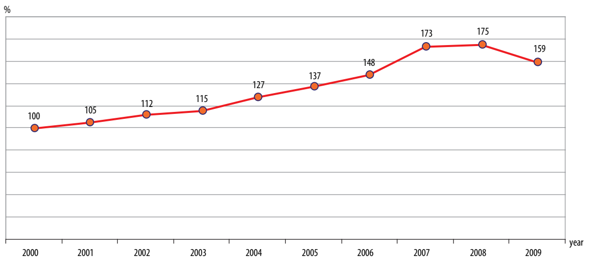
Fig. 2. The dynamics of changes in traffic volume on all main, national and partly regional Lithuanian roads for the period 2000–2009
