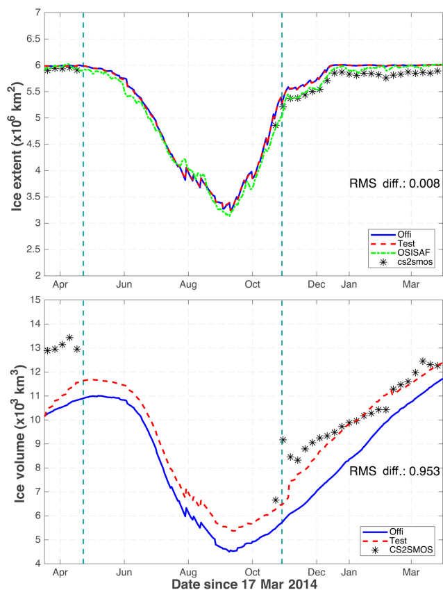
Figure 11. SIE and SIV in the official run (blue) and the test run (red) in the Central Arctic. The black stars are the corresponding weekly SIE (or SIV) estimated from CS2SMOS. The green dashed line is the daily SIE from OSI-SAF. The averaged differences of the two runs (Official–Test) are reported. The vertical cyan dashes delimits the periods when C2SMOS data is assimilated.
