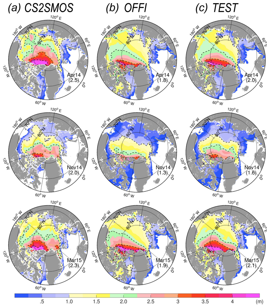
Figure 3. Monthly SIT from CS2SMOS, column (a), Official run, column (b), and Test run, column (c) in April 2014, November 2014, and March 2015, respectively. The mean SIT estimated for the area north of 80° N is indicated between parentheses (unit: m). The dashed lines are isolines of 1, 2, 3 and 4 m SIT, respectively.
