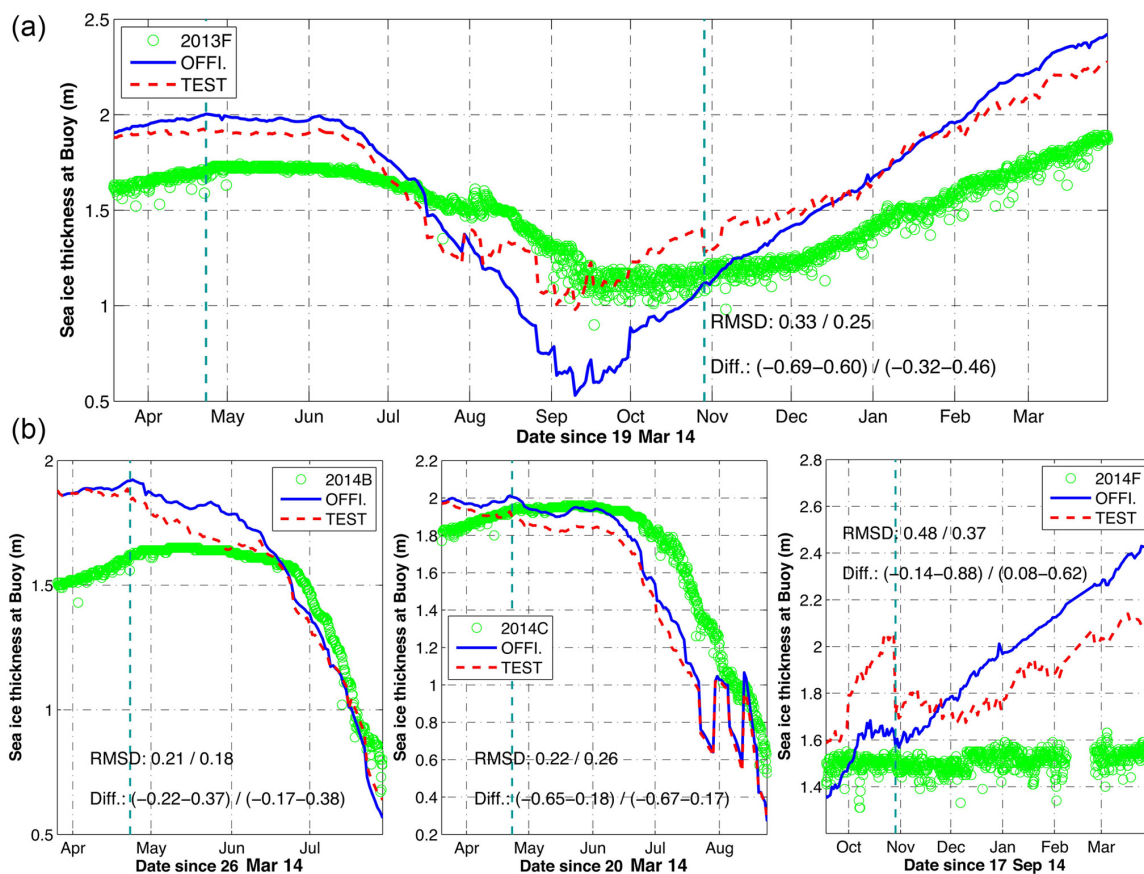
Figure 5. Time series of SIT along the trajectories of IMB buoys (a: 2013F; b: 2014B, 2014C and 2014F). Measured SIT (green), daily averages from the Official run (blue line) and the Test run (red line). The vertical cyan-dashed lines indicate the winter period when C2SMOS is assimilated in the Test run.
