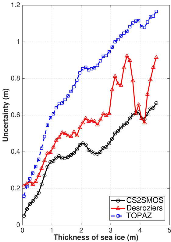
Figure 2. Observation error uncertainties as a function of sea-ice thickness for the original CS2SMOS data set (black line), the estimated observation error using the Desroziers diagnostics with red-triangle line (see Eq. 3) and the one used in the TOPAZ Test run with blue-square, with an additional error term as Eq. (4) to the original uncertainty.
