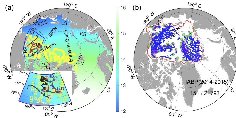
Figure 1. (a) Horizontal resolution (km) of the model grid in the Arctic ( > 60^\circ \text{N} ). The small yellow squares are the locations of IceBridge campaigns during the experimental period. The marginal seas are as follows: Beaufort Sea (BS; also shown with the blue line), Chukchi Sea (CS), East Siberian Sea (ESS), Laptev Sea (LS) and Kara Sea (KS); and the other regions are as follows: Canadian Arctic Archipelago (CAA), Svalbard Island (SI) and Fram Strait (FM). The four purple markers (star, circle, triangle and diamond) are the deployment location of IMB buoys (2013F, 2014B, 2014C, and 2014F respectively) with the following trajectory shown as black solid curves. The three red squares are the fixed locations of the BGEF moorings (14A, 14B and 14D, respectively). (b) Trajectories of International Arctic Buoy Program buoys drift during the experimental period. The solid red line delimits the coastal areas excluded in the analysis.
