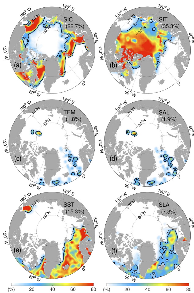
Figure 13. Relative DFS contributions (IF) of each observation data types in November 2014. (a) SIC from OSI-SAF; (b) SIT from CS2SMOS; (c) temperature profiles; (d) salinity profiles; (e) SST; (f) along-track sea level anomaly (SLA). The black line is the 20 % isoline, and the monthly IF (see Eq. 12) is reported between parentheses.
