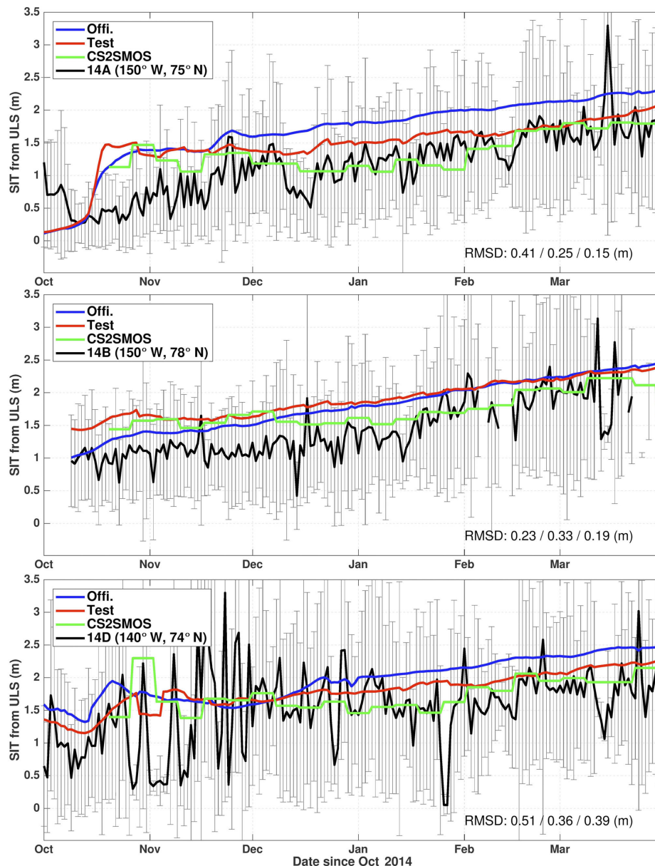
Figure 6. Daily series of SIT (black line) at the BGEP mooring (14A, 14B, and 14D) compared with the two model runs – Official (blue line) and Test (red line) – and the weekly observed by CS2SMOS (green line). The black line represents the daily average at the mooring location with the standard deviation shown as the error bar. The RMSDs of the Official run, Test run and CS2SMOS are respectively indicated on the bottom of each panels.
