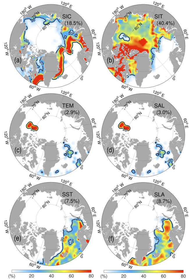
Figure 14. Same as the above but for March 2015.
