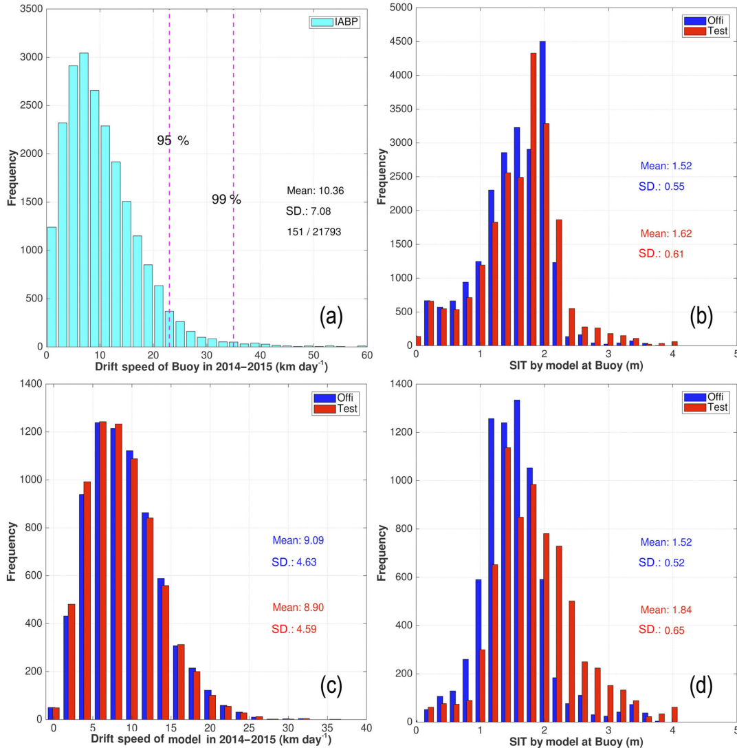
Figure 10. (a) Histogram of sea-ice drift speeds calculated from IABP buoys in the Central Arctic for the period 2014–2015. (b) histogram of the simulated SIT at buoys locations in the Central Arctic from the two runs. (c) histogram of the drift speed restricted near the North Pole (> 80° N) in the Official (blue) and Test (red) runs; the mean speed and the standard deviation are indicated; (d) histogram of the simulated SIT near the North Pole from the two runs.
