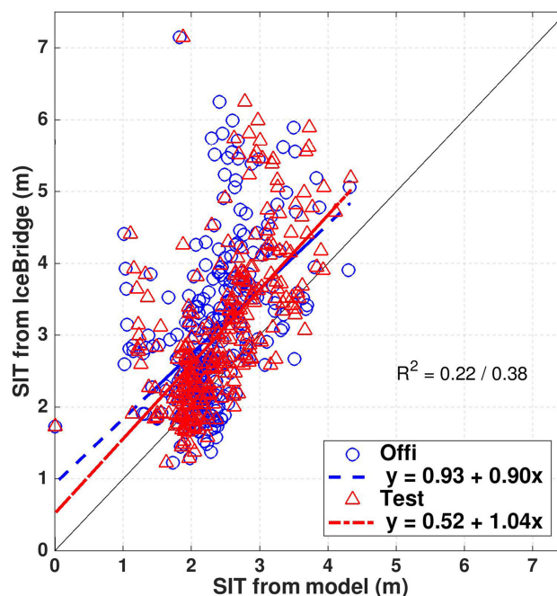
Figure 8. Scatterplots of SIT daily averaged of Official (blue) and Test (red) runs compared to IceBridge data. The dashed lines are the respective linear regression, the coefficient R^2 is the squared correlation to represent how strong of the linear relationship in Official or Test run. The black line is y = x .
