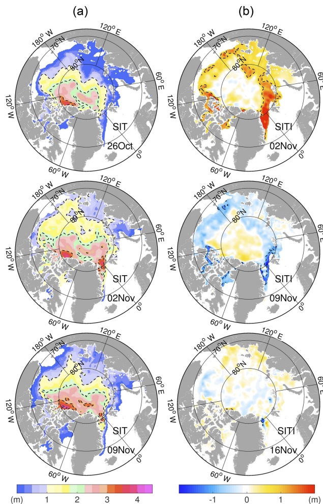
Figure 12. (a) First three weekly SITs (20–26 October; 27 October–2 November; 3–9 November) from CS2SMOS in the beginning of fall 2014. The dashed white lines denote the 1, 2, 3 and 4 m isolines. (b) The associated time increments of SIT relative to the last weekly SIT. The dashed isolines denote \pm 1 m.
