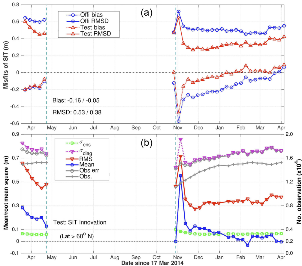
Figure 4. (a) Bias (dotted line) and RMSD (solid line) of SIT in the two runs – Official (blue) and Test (red) – based on weekly averaged reanalysis and CS2SMOS observations. The time-averaged bias and RMSD are indicated (Official/Test). (b) SIT innovation statistics in the Test run in the Arctic region (> 60° N) from 19 March 2014 to end of March 2015. The blue-squared (red reverted-triangle) line represents the mean (RMSD) of the innovation. The green squared line represents the ensemble spread and the purple reverted-triangle line is the diagnosed total uncertainty (see Eq. 8). The gray-crossed (gray-circled) line is the number (RMSD observation error) of assimilated observations.
