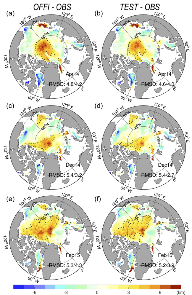
Figure 9. Sea-ice drift misfits (model minus observation, in km per 2 days) in the Official run (a, c, e) and Test run (b, d, f), compared against the OSI-SAF sea-ice drift in April 2014 (a, b), December 2014 (c, d) and February 2015 (e, f). The black dashed line delimits the area of fastest drift (drift > 3 \text{ km per 2 days} ), and the RMSD relative to the monthly observations is indicated when calculated for the whole domain and at for the region north of 80^\circ \text{ N} .
