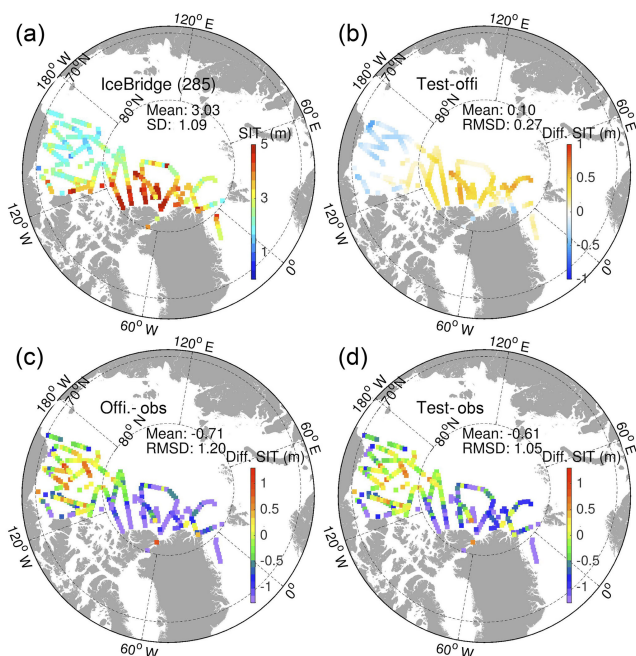
Figure 7. (a) IceBridge SIT in 2014 and 2015 and (b) the SIT differences in the two model runs according to the observational locations and times. SIT deviations (c, d) from the Official run (c) and Test run (d) using model daily average at observations time.
