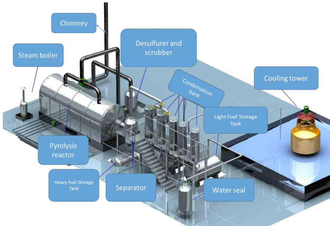
FIG. 3. Components of the pilot pyrolysis plant.
