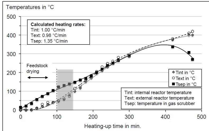
FIG. 5. Reactor heating curve [10].
