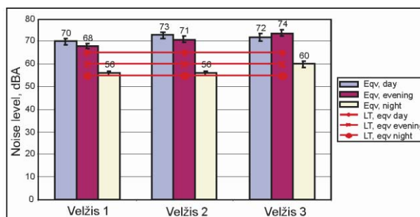
Fig. 2. Dynamics of equivalent noise levels in Velžis street within twenty four hours
