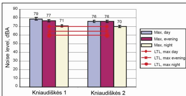
Fig. 29. Dynamics of maximum noise levels in Kniaudiškės street within twenty four hours
