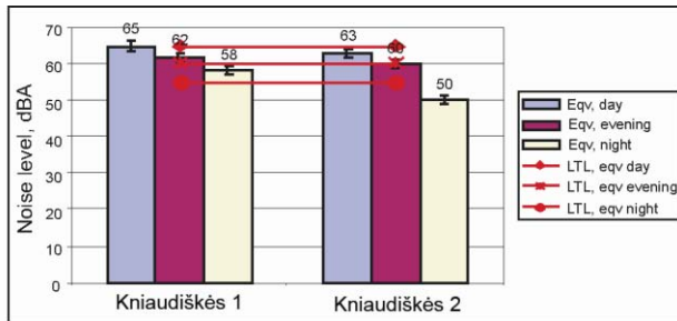
Fig. 28. Dynamics of equivalent noise levels in Kniaudiškės street within twenty four hours
