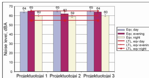
Fig. 16. Dynamics of equivalent noise levels in Projektuotojai street within twenty four hours
