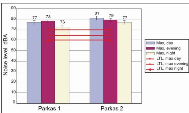
Fig. 19. Dynamics of maximum noise levels in Parkas street within twenty four hours
