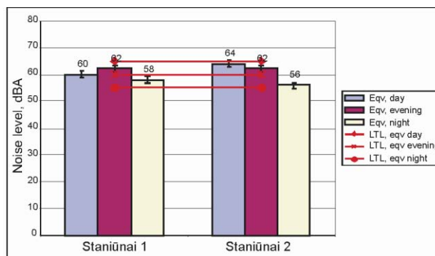
Fig. 24. Dynamics of equivalent noise levels in Staniūnai street within twenty four hours
