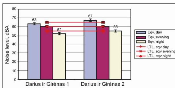
Fig. 26. Dynamics of equivalent noise levels in Darius and Girėnas street within twenty four hours
