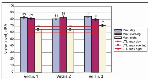
Fig. 3. Dynamics of maximum noise levels in Velžis street within twenty four hours
