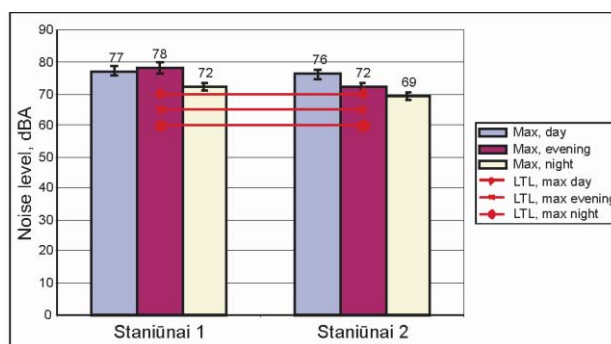
Fig. 25. Dynamics of maximum noise levels in Staniūnai street within twenty four hours
