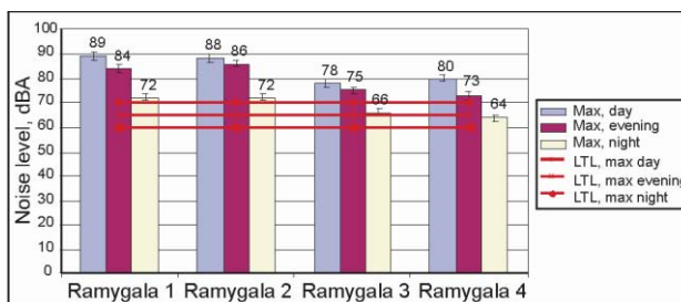
Fig. 7. Dynamics of maximum noise levels in Ramygalą street within twenty four hours
