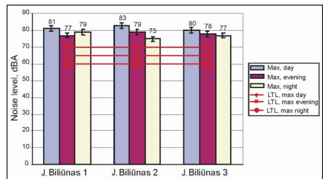
Fig. 21. Dynamics of maximum noise levels in J. Biliūnas street within twenty four hours
