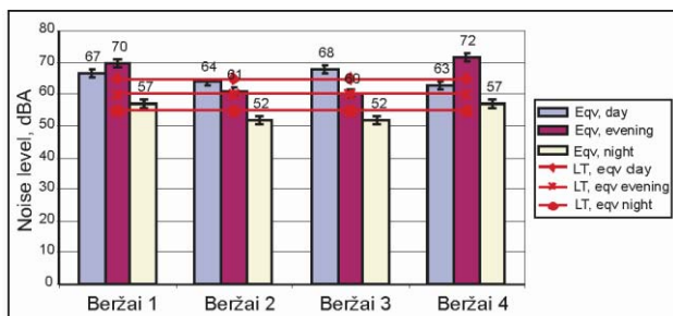
Fig. 4. Dynamics of equivalent noise levels in Beržai street within twenty four hours
