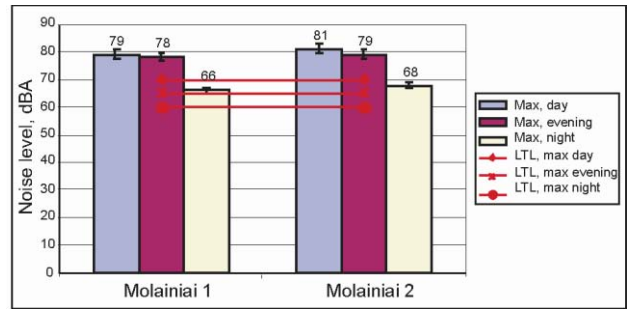
Fig. 11. Dynamics of maximum noise levels in Molainiai street within twenty four hours
