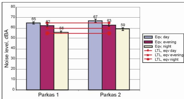
Fig. 18. Dynamics of equivalent noise levels in Parkas street within twenty four hours
