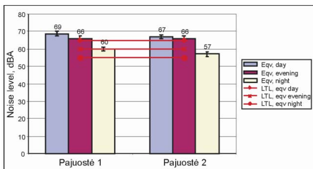
Fig. 22. Dynamics of equivalent noise levels in Pajuostė street within twenty four hours
