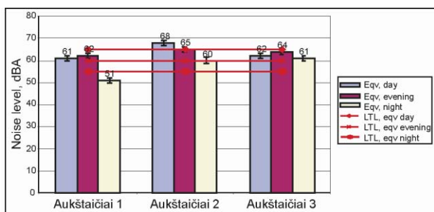
Fig. 14. Dynamics of equivalent noise levels in Aukštaičiai street within twenty four hours
