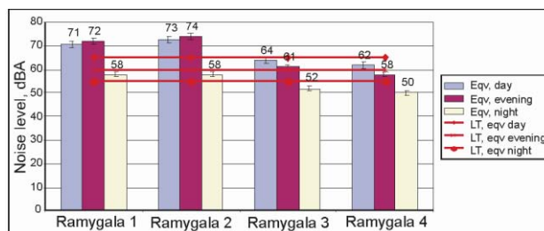
Fig. 6. Dynamics of equivalent noise levels in Ramygalą street within twenty four hours
