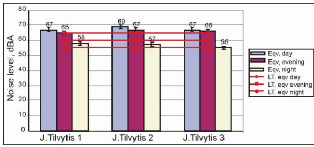
Fig. 8. Dynamics of equivalent noise levels in J. Tilvytis street within twenty four hours
