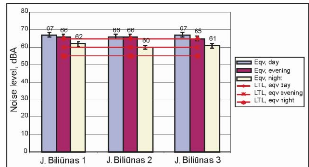
Fig. 20. Dynamics of equivalent noise levels in J. Biliūnas street within twenty four hours
