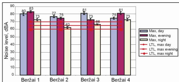
Fig. 5. Dynamics of maximum noise levels in Beržai street within twenty four hours
