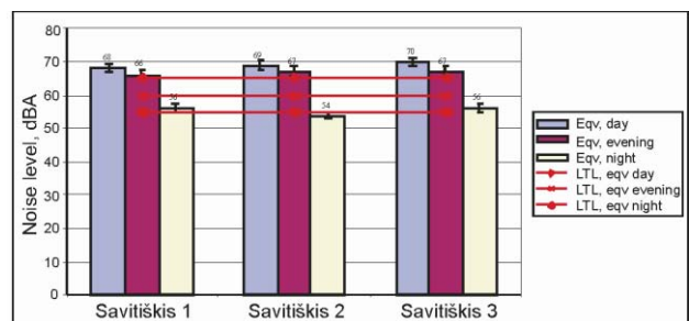
Fig. 12. Dynamics of equivalent noise levels in Savitiškis street within twenty four hours
