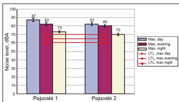
Fig. 23. Dynamics of maximum noise levels in Pajuostė street within twenty four hours
