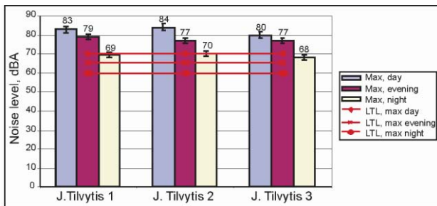
Fig. 9. Dynamics of maximum noise levels in J. Tilvytis street within twenty four hours
