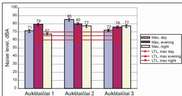
Fig. 15. Dynamics of maximum noise levels in Aukštaičiai street within twenty four hours
