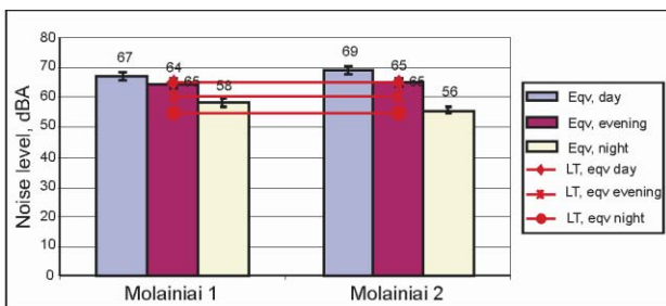
Fig. 10. Dynamics of equivalent noise levels in Molainiai street within twenty four hours
