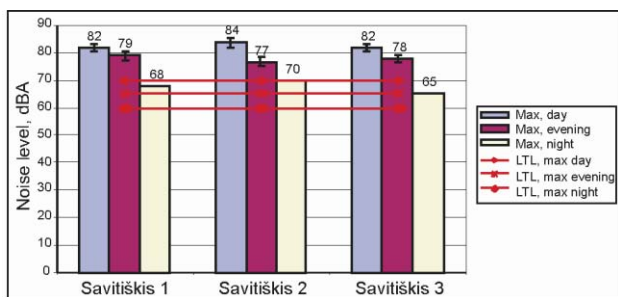
Fig. 13. Dynamics of maximum noise levels in Savitiškis street within twenty four hours
