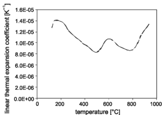
Fig. 4. Linear thermal expansion coefficient as a function of temperature
