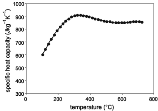
Fig. 2. Specific heat capacity as a function of temperature
