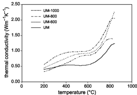
Fig. 3. Thermal conductivity as a function of temperature
