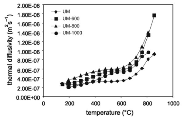
Fig. 1. Thermal diffusivity as a function of temperature
