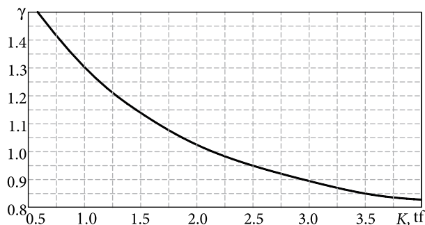
Fig. 2. Nomogram of empirical coefficient \gamma
