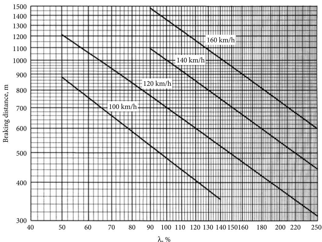
Fig. 1. Assessment graphics of the braked mass percentage \lambda of passenger wagons
