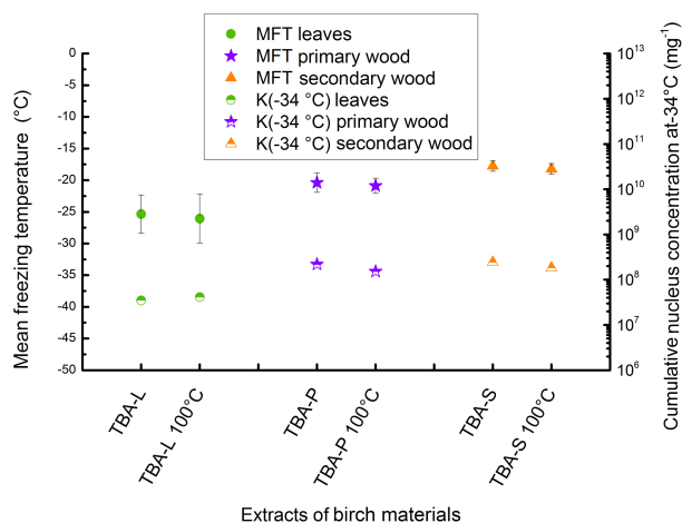
Figure 6. Results of the heat treatment of the different TBA extracts. Leaves are marked with green circles, primary wood with violet stars, and secondary wood with orange triangles. The left value belongs to the untreated sample, the right value to the sample treated with 100 °C for 1 h. Filled symbols represent the mean freezing temperature and correlate with the left y axis; half-filled symbols represent the cumulative nucleus concentration as -34\text{ }^{\circ}\text{C mg}^{-1} extracted sample and correlate with the right y axis.
