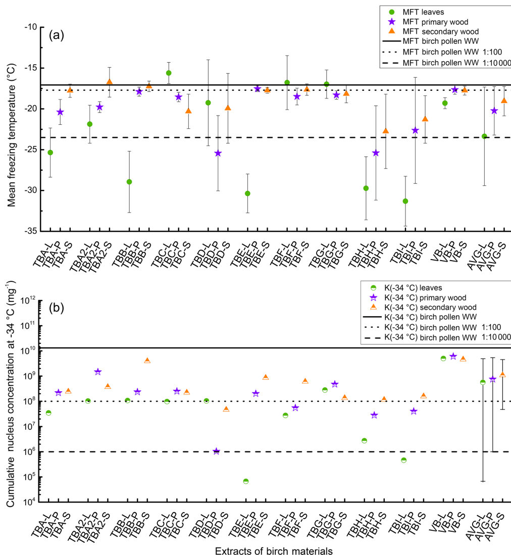
Figure 2. (a) Mean freezing temperature (MFT) of the different birch samples. Leaf extracts (L) are marked with green circles, primary wood extracts (P) with violet stars, and secondary wood extracts (S) with orange triangles. The solid line is the MFT of birch pollen washing water ( -17.1^{\circ}\text{C} with a standard deviation of \pm 0.5^{\circ}\text{C} (not plotted)). The dotted line represents the MFT of a dilution equivalent to 10^8 INP \text{mg}^{-1} ( -17.7^{\circ}\text{C} with a standard deviation of \pm 1.1^{\circ}\text{C} (not plotted)) and the dashed line refers to the MFT of a dilution equivalent to 10^6 INP \text{mg}^{-1} ( -23.5^{\circ}\text{C} with a standard deviation of \pm 3.6^{\circ}\text{C} (not plotted)). The three values on the far right side of (a) represent the average of all mean freezing temperatures for leaves (AVG-L), primary wood (AVG-P), and secondary wood (AVG-S) with the corresponding standard deviation. (b) Cumulative nucleus concentration at -34^{\circ}\text{C} ( K(-34^{\circ}\text{C}) ) of the different birch samples \text{mg}^{-1} extracted sample. Assignment of the symbols is similar to the top plot. The solid line refers to the K(-34^{\circ}\text{C}) of birch pollen washing water \text{mg}^{-1} extracted pollen ( 1.3 \times 10^{10} \text{ mg}^{-1} ); the dotted and dashed line refer to the dilutions from birch pollen washing water introduced in (a). The three values on the far right side represent the average of all K(-34^{\circ}\text{C}) values. Error bars point to the area of trust, ranging from the highest to the lowest measured values.
