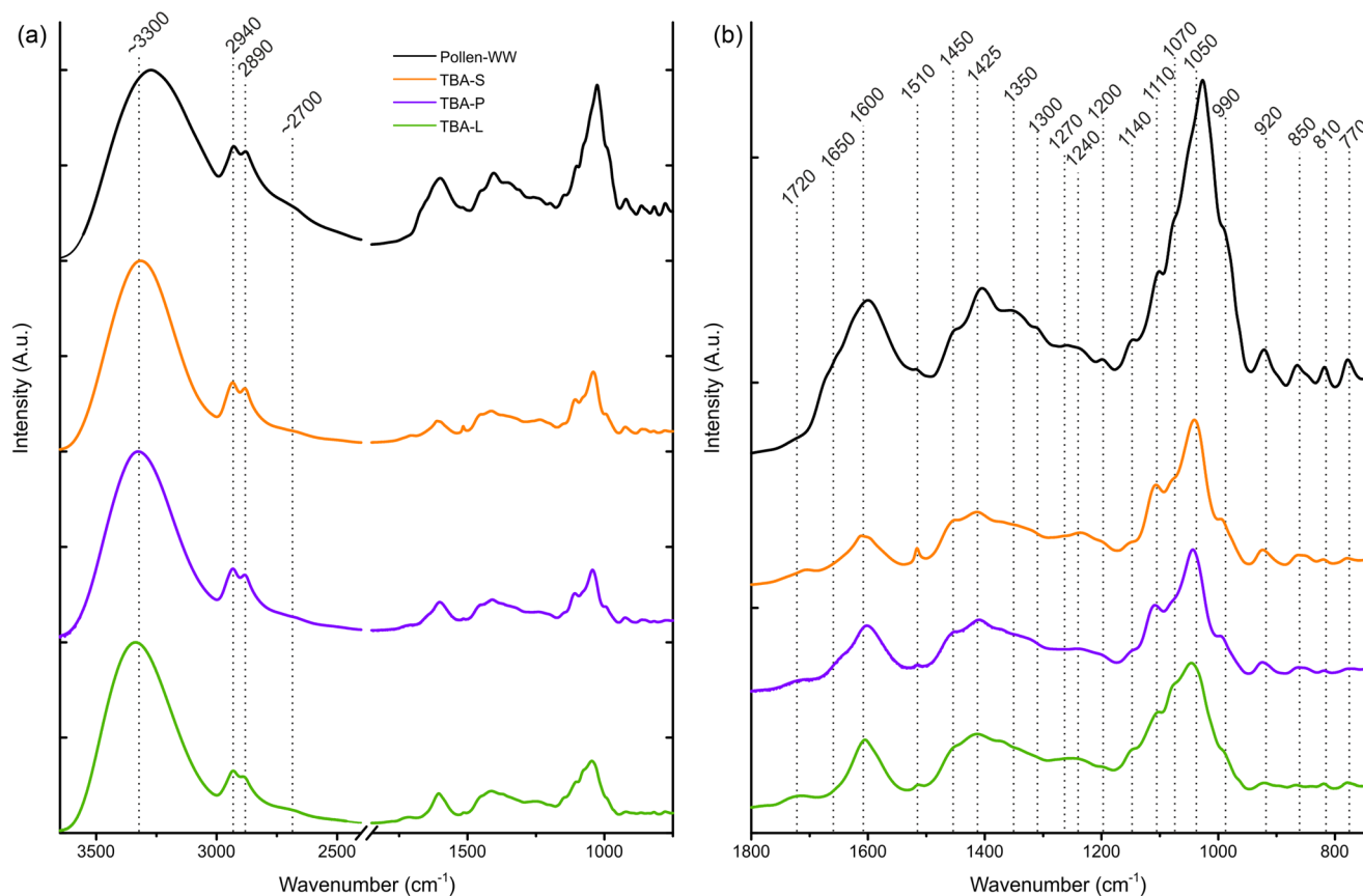
Figure 7. FTIR spectra of the TBA extracts (leaves in green, primary wood in violet, and secondary wood in orange) and birch pollen washing water (black). (a) The whole spectrum between 3650 and 750 \text{cm}^{-1} . (b) Enlarged right side of the spectrum between 1800 and 750 \text{cm}^{-1} . Possible band assignments are given in Table 3.
