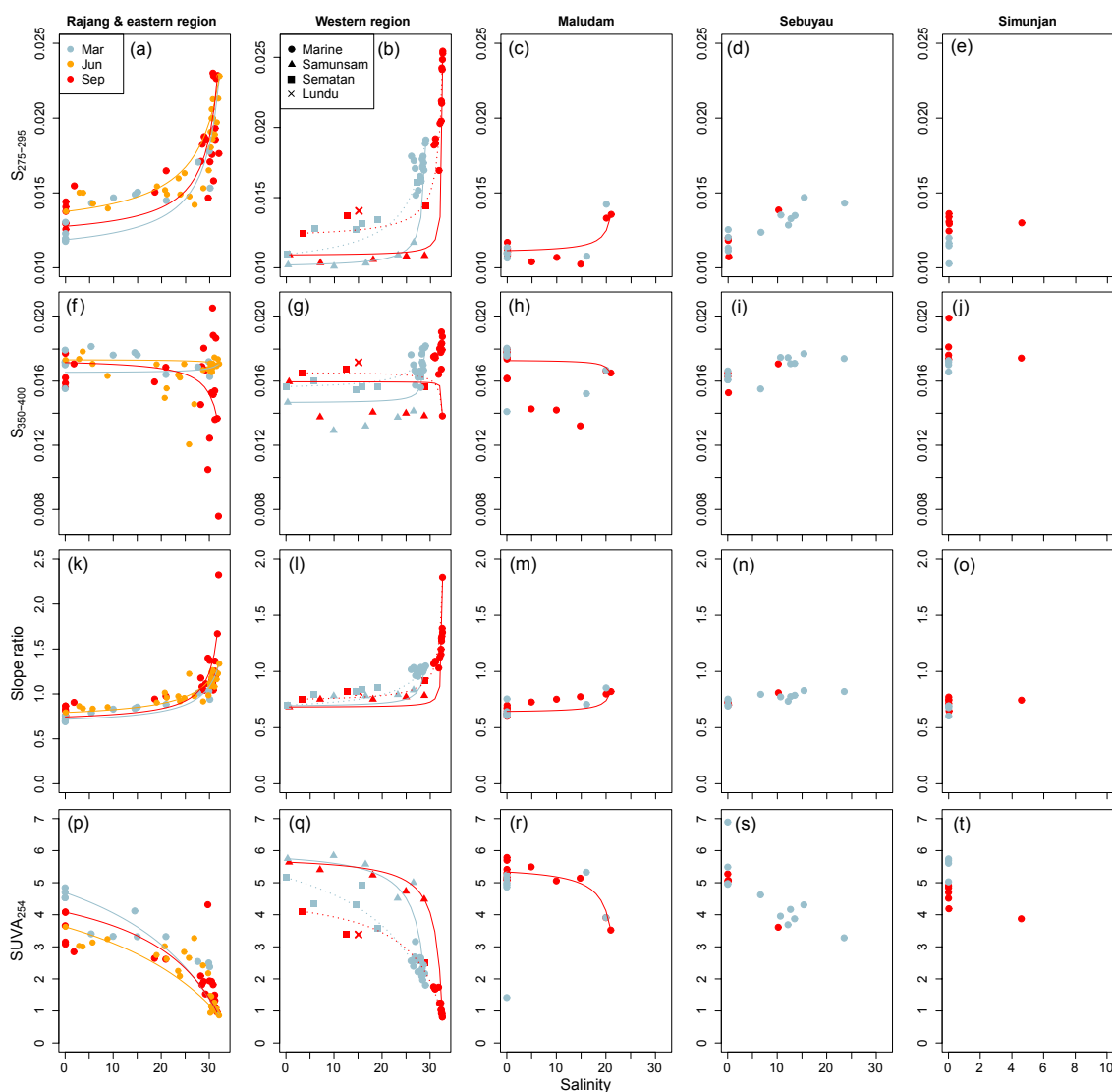
Figure 4. Changes in (a–e) S_{275-295} , (f–j) S_{350-400} , (k–o) CDOM spectral slope ratio, and (p–t) SUVA_{254} from rivers to coastal seawater. Conservative mixing lines are shown as in Fig. 2 (note that conservative mixing of CDOM properties is non-linear). Data are shown separately for each sampling region as indicated by column titles.
