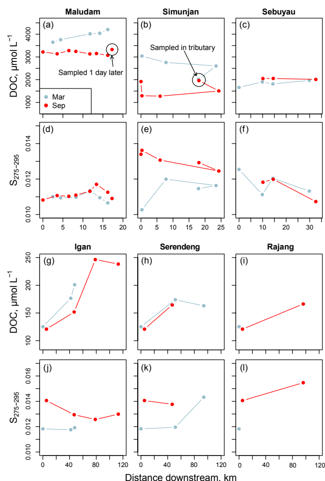
Figure 3. Changes in (a–c) and (g–i) dissolved organic carbon concentration and (d–f) and (j–l) S_{275-295} with distance downstream for all stations with salinity of 0. Data in (a–f) are for the Maludam, Simunjan, and Sebuyau rivers, while (g–l) show data for the three main Rajang distributaries (named in Fig. 1b): panels (h, k) show data for the Serendeng branch (includes the Lebaan and Paloh sections), while panels (i, l) show data for the Rajang branch (includes the Payang section).
