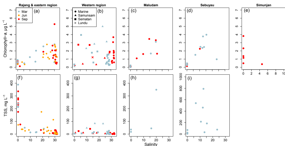
Figure 7. Distribution of (a–e) chlorophyll- a , and (f–i) total suspended solids from rivers to coastal seawater for each study region. TSS was not measured in the Simunjan.
