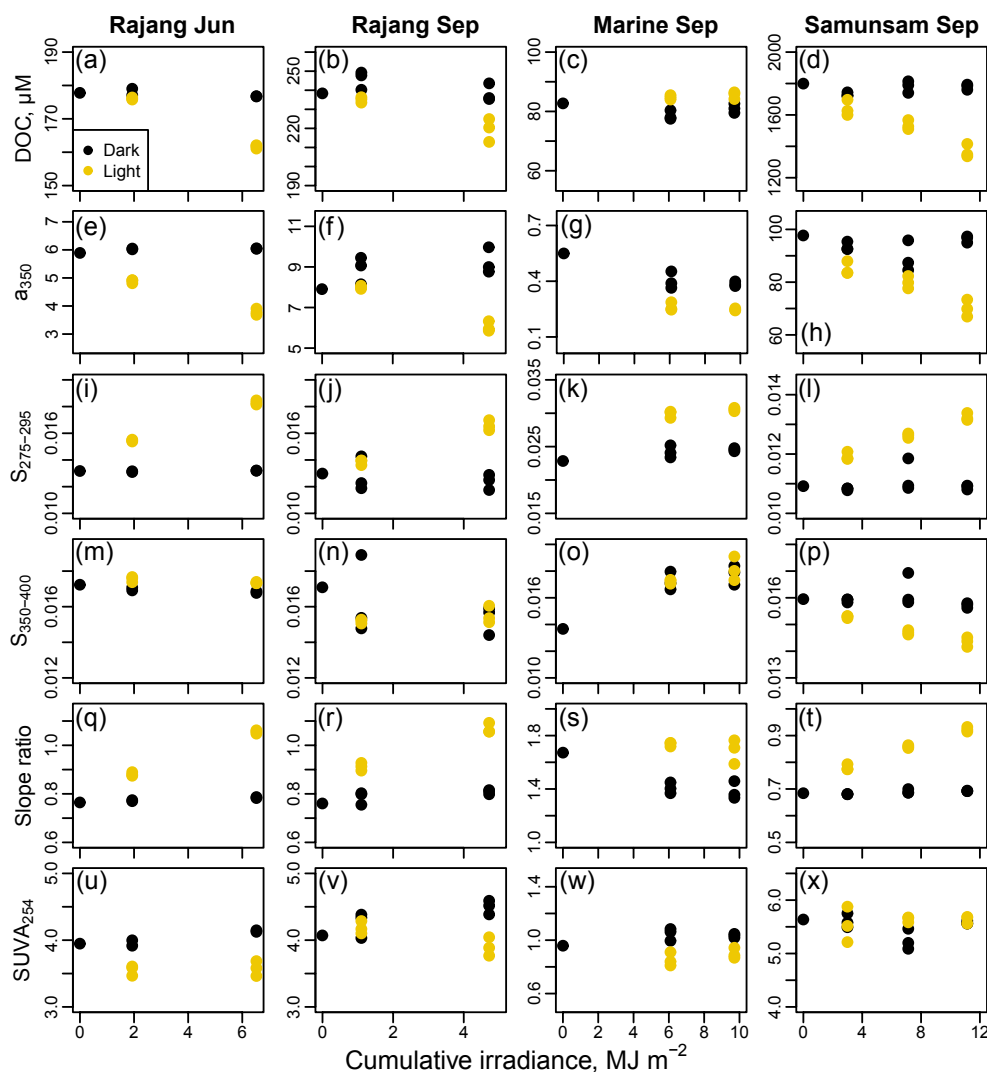
Figure 6. Results from photodegradation experiments showing the decrease in DOC (a–d), CDOM concentration (e–h), S_{275-295} (i–l), S_{350-400} (m–p), CDOM spectral slope ratio (q–t), and SUVA_{254} (u–x) with cumulative irradiance from 318 to 450 nm in wavelength. Each column corresponds to one degradation experiment, as indicated in the column titles. Black symbols indicate dark control bottles; yellow symbols indicate light-exposed bottles.
