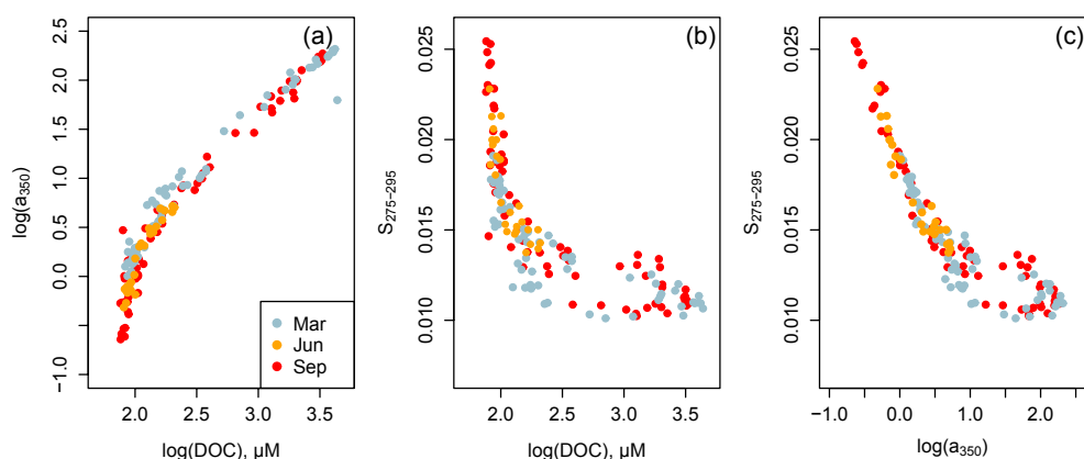
Figure 5. Scatter plots of (a) CDOM absorption versus DOC concentration, (b) S_{275-295} versus DOC concentration, and (c) S_{275-295} versus CDOM absorption for the entire data set. Strong relationships were found between these parameters but without seasonal variation.
