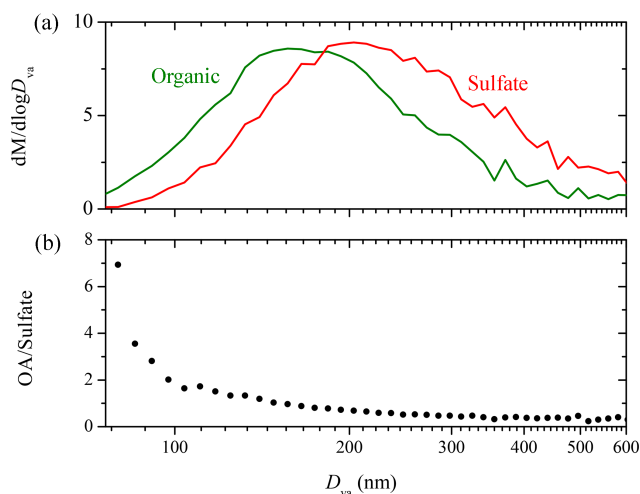
Figure 7. (a) The AMS-measured organic (green) and sulfate (red) mass distribution ( D_{va} from 75 to 600 nm) for Exp. 4; (b) the dependence of the AMS-derived organic to sulfate ratio on particle vacuum aerodynamic diameter (75–600 nm). The results are based on particle time-of-flight data averaged over \sim 1.4 h ( t = 2.1 – 3.5 h).
