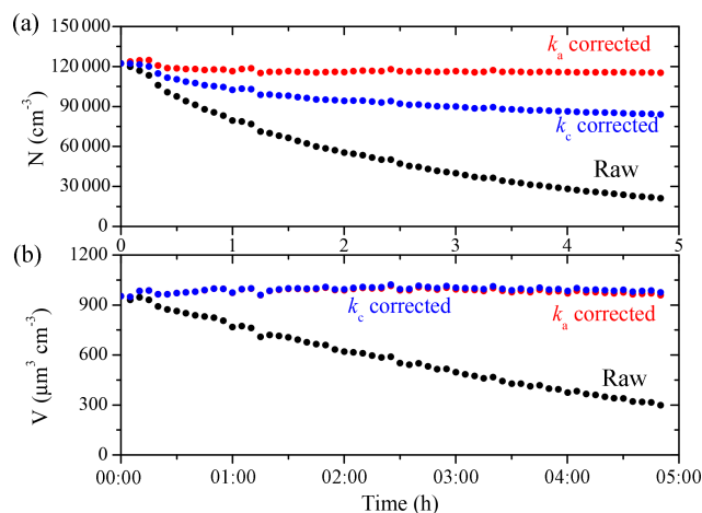
Figure 2. The SMPS-measured (black symbols) and the particle-wall-loss-corrected (a) number and (b) volume concentration using the k_a(D_p) profile (red symbols) and the k_c(D_p) profile (blue symbols) for Exp. 1.
