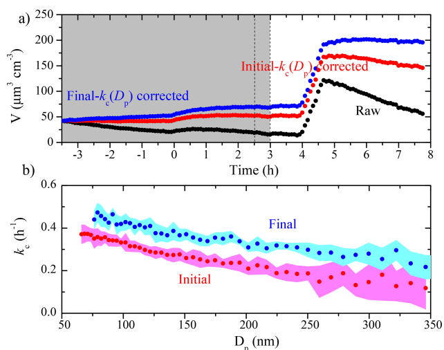
Figure 8. (a) The SMPS-measured (black symbols), the initial k_c(D_p) -corrected (red symbols), and the final k_c(D_p) -corrected (blue symbols) particle volume concentration time series for an aging experiment (Exp. 5), together with (b) the initial (red symbols) and the final (blue symbols) k_c(D_p) profiles. The colored areas are the uncertainties associated with the corresponding k_c(D_p) . The grey area indicates that the chamber was dark. The two dashed lines mark the beginning and the end of HONO addition into the chamber. Ammonium sulfate seed particles were injected into the chamber at t = 4 h.
