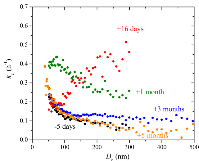
Figure 9. The coagulation-corrected particle wall-loss rate constant, k_c , at each diameter derived from experiments with only ammonium sulfate particles in the 12 \text{ m}^3 CMU Teflon chamber before and after some major maintenance in the room where the chamber is suspended. The chamber was partially deflated and its walls subjected to friction repeatedly during the maintenance.
