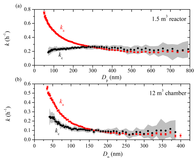
Figure 1. The apparent (red symbols) and coagulation-corrected (black symbols) particle wall-loss rate constants as a function of particle size for (a) the 1.5 m 3 Teflon reactor and (b) the 12 m 3 CMU smog chamber after the two systems have been left undisturbed in the lab for weeks. The particle loss rate constants were derived based on SMPS measurements from Exp. 1 and 2. Only k_a values with an R^2 > 0.5 are shown. The error bars correspond to 1 standard deviation. The grey area is the uncertainty associated with k_c .
