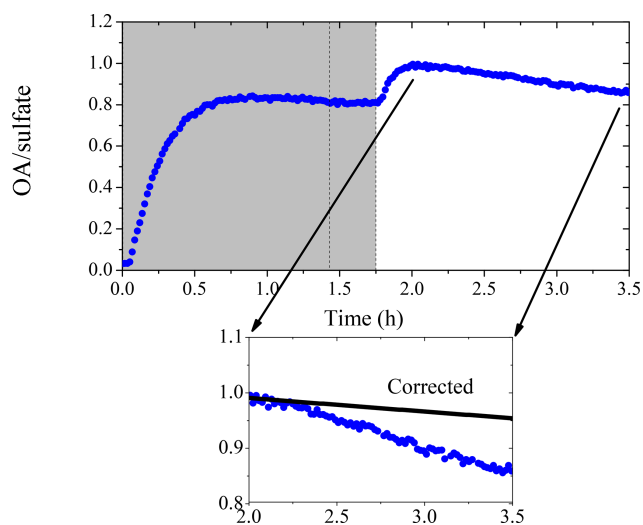
Figure 6. The organic to sulfate ratio time series derived from AMS measurements for Exp. 4 (data after the second HONO introduction are not shown). The inset is a blow-up of the OA / sulfate ratio from its maximum until the second HONO introduction. The black symbols are the size-dependence-corrected OA / sulfate during that 1.5 h. The shaded area indicates that the chamber was dark. The dashed lines mark the beginning and the end of the first HONO injection into the chamber.
