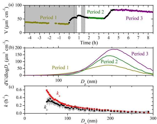
Figure 4. (a) The SMPS-measured particle volume concentration time series for an aging experiment (Exp. 3) with three colored periods used to derive the corresponding size-independent particle wall-loss rate constants, k_1 – k_3 (Eq. 2). The grey area indicates that the chamber was dark. The dashed lines mark the beginning and the end of bubbling HONO into the chamber twice; (b) the averaged particle volume size distribution over the three periods used to develop k_1 – k_3 based on the SMPS measurement for Exp. 3; (c) the size-dependent particle wall-loss rate constants determined from SMPS-measured particle number concentration from Period 1 for Exp. 3. Only k_a values (red symbols) with an R^2 > 0.5 are shown. The error bars correspond to \pm 1 standard deviation. The grey area is the uncertainty associated with k_c (black symbols).
