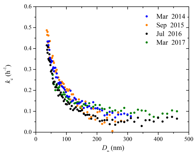
Figure 3. The k_c(D_p) profiles for the 12\text{ m}^3 CMU Teflon chamber over a span of 3 years. The particle wall-loss rate constants were derived based on SMPS measurements from experiments with only ammonium sulfate particles.
