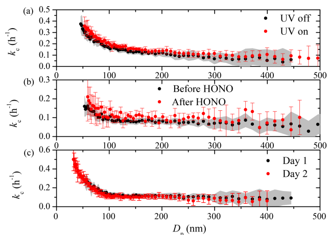
Figure 10. The coagulation-corrected particle wall-loss rate constant, k_c , at each diameter for (a) Exp. 6, (b) Exp. 7, and (c) Exp. 8 and 9. The uncertainties associated with the corresponding k_c(D_p) values are either expressed as the grey area or the red error bars.
