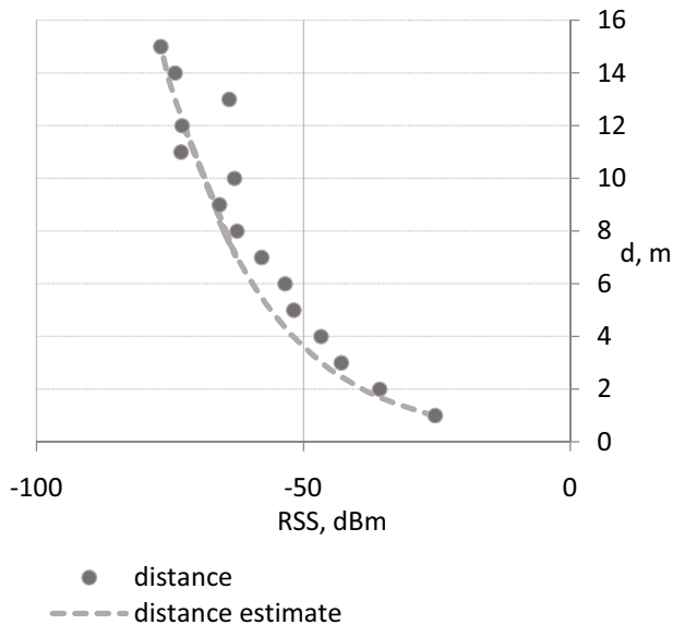
Fig. 2. Estimated and real distances between access point and mobile device
