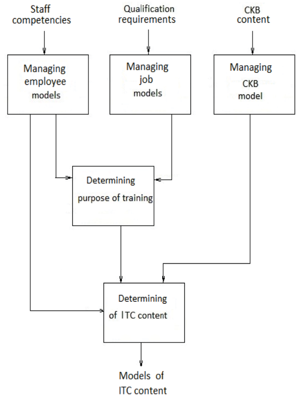
Fig. 2. Context diagram decomposition
