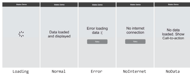
Fig. 11. Screen states
