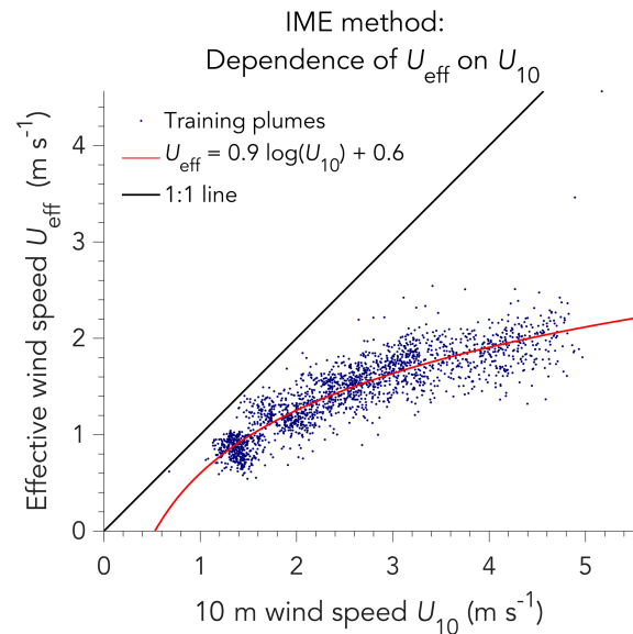
Figure 4. Relationship between the effective and local 10 m wind speeds in the IME method, characterized with LES training plumes assuming 1% instrument precision. Each point represents a different LES plume pseudo-observation from the training set. The red line fits the data to a logarithmic dependence. The 1 : 1 line is shown in black. See text for similar results with 3% or 5% instrument precision.
