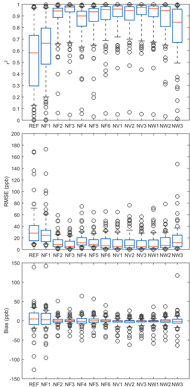
Figure 4. FLEXPART CTM model performance based on boxplots of coefficient of determination, root mean square error (RMSE) and bias in daily average methane model fractions at surface stations for different kernel settings (see Table 1). Independent validation stations are included. The red line in the boxplots indicates the median, the bottom and top box edges are the 25th and 75th percentiles, and whisker ends are at 9th and 91st percentiles. The circles are outliers.
