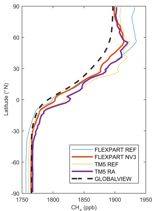
Figure 10. Zonal mean surface methane (ppb) in 2013 based on FLEXPART CTM, TM5 and GLOBALVIEW-CH 4 .
