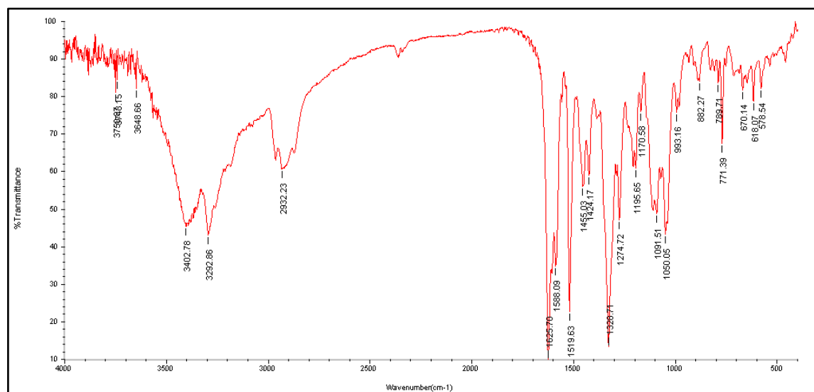
Figure 11. FTIR Spectrum of pure ticagrelor powder
