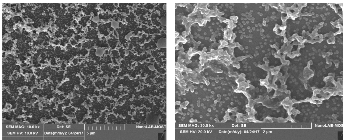
Figure 20. Scanning electron microscope image of F12 (HPMC) nanoparticles at different magnification
