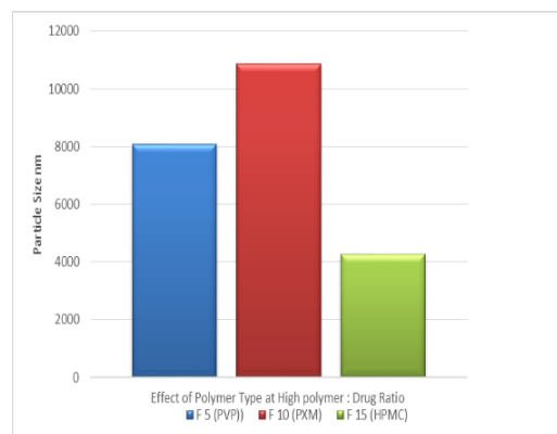
Figure 10. Effect of polymer type at high solvent:antisolvent ratio (1: 15) on nanoparticles size
