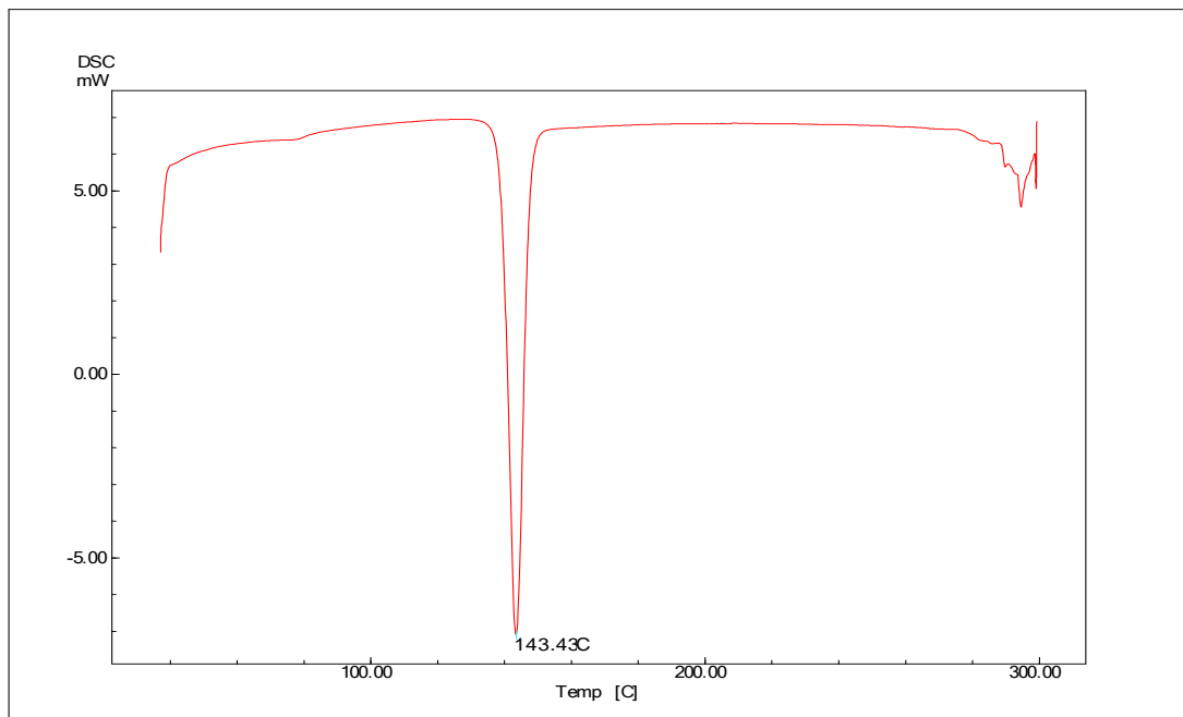
Figure 13. DSC thermogram of pure ticagrelor
