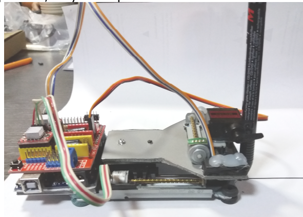
Figure 3. Experimental tests with the 2-axis CNC pen plotter
