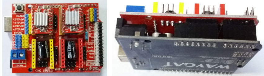
Figure 2. Electrical and physical coupling between Arduino and driver module
