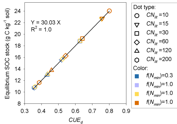
Figure A4. Relationship between C stock of the potentially equilibrated SOM pool and the carbon use efficiency of decomposed metabolic litter ( CUE_d ) at the dynamic equilibrium stage. f(N_{min}) denotes the inhibition factor (0–1) of soil mineral N on litter decomposition.
