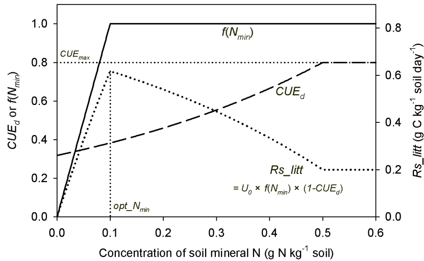
Figure A5. Schematic plot for change trends of f(N_{min}) (inhibition effect of mineral N; Eq. 6), CUE_d (carbon use efficiency of decomposed litter; Eqs. 2, 3) and Rs_{litt} (litter respiration rate) with increasing concentration of soil mineral N. CUE_{max} (equal to 0.8) is the maximum CUE set in this study. opt\_N_{min} denotes the concentration of soil mineral N at which litter respiration is maximized. U_0 is the potential decomposition rate when mineral N is fully adequate for litter decay.
