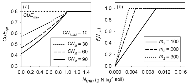
Figure 2. Schematic plot of (a) the optimal carbon use efficiency (CUE opt ) as a function of soil mineral nitrogen for different litter C : N ratios (from Eq. 2) in the main text (with m_1 = 0.3 , n_1 = 1.0 ) and (b) the N limitation function f(N_{\min}) applied to litter decomposition rates (from Eq. 5) in the main text. CN_{\text{lit}} and CN_{\text{SOM}} are the C : N ratios of the litter and SOM pools, respectively. CUE_{\text{max}} = 0.8 is the maximum CUE under optimal nutrient condition (C limitation only). m_1 and n_1 are the parameters of Eq. (3) and m_2 is the parameter of Eq. (5).
