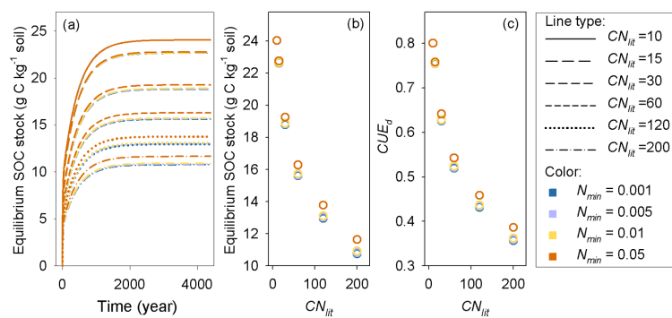
Figure 7. (a) Accumulation of soil organic carbon (SOC) for constant substrates input (plant litter) with different C : N ratios ( CN_{lit} ) at different levels of soil mineral N concentrations ( N_{min} , g\ N\ kg^{-1} soil), (b) change trends of equilibrium SOC stock and (c) carbon use efficiency of decomposed litter ( CUE_d ) with increasing litter C : N ratio.
