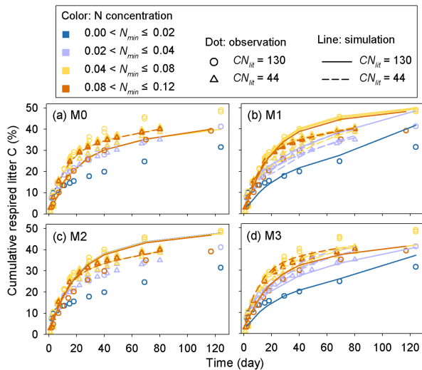
Figure 5. Time series of the simulated (lines) and observed (dots) cumulative respired litter C (% of initial litter C) at four different levels of soil mineral N availability ( N_{min} , \text{g N kg}^{-1} soil). CN_{lit} is the C : N ratio of plant litter. M0–M3 denote the four models tested in this study (Table 1). Here, the simulation results of each model were calculated with parameters optimized based on all of the 14 samples of incubation experiments (Table A2).
