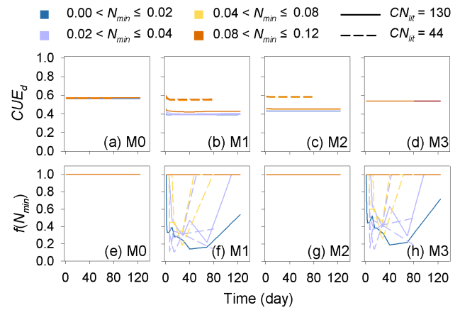
Figure A3. Dynamic of the simulated carbon use efficiency (CUE) and f(N_{min}) during the incubation experiments (Table A4). CN_{lit} is the C : N ratio of incubated litter, and N_{min} is the initial soil mineral N concentration ( g\ N\ kg^{-1} soil). M0–M3 are the four models in Table 1. Here, the simulation results of each model were calculated with parameters optimized based on all of the 14 samples of incubation experiments (Table A2).
