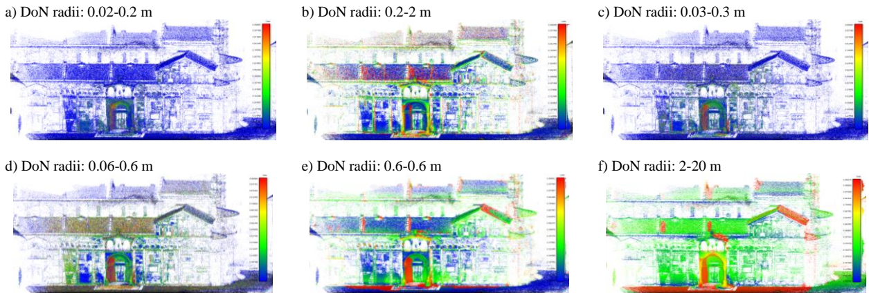
Figure 5: Vector magnitude of the Difference of Normals (DoN) operator using several combination of radii. The DoN operator produces high response in areas with significant surface changes in the given radii range. For small radii values (i.e. case a ), greater variations are expected in fine-detailed areas. Increasing the radii values (i.e. case f ), DoN detects higher changes in the large architectural parts (roof, façade,..).
