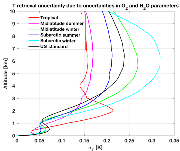
Figure 10. Uncertainty in temperature retrievals from ground-based MWR due to the uncertainty in \text{O}_2 and \text{H}_2\text{O} absorption model parameters. The observation vector considered here consists of T_{\text{B}} at the 14 HATPRO channels. Six climatological atmospheric conditions (color coded) have been used to compute K_{\text{b}} and K_{\text{x}} . The square roots of the diagonal terms of \text{Cov}_{\text{p}} are shown. 101 pressure levels from 0.005 to 1050 hPa are used here. These levels have been selected specifically to be denser close to the surface (34 levels below 2 km). The vertical spacing of levels is given in Fig. 1 of De Angelis et al. (2016).
