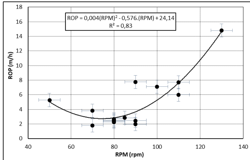
Figure 2. ROP-RPM relationship diagram
