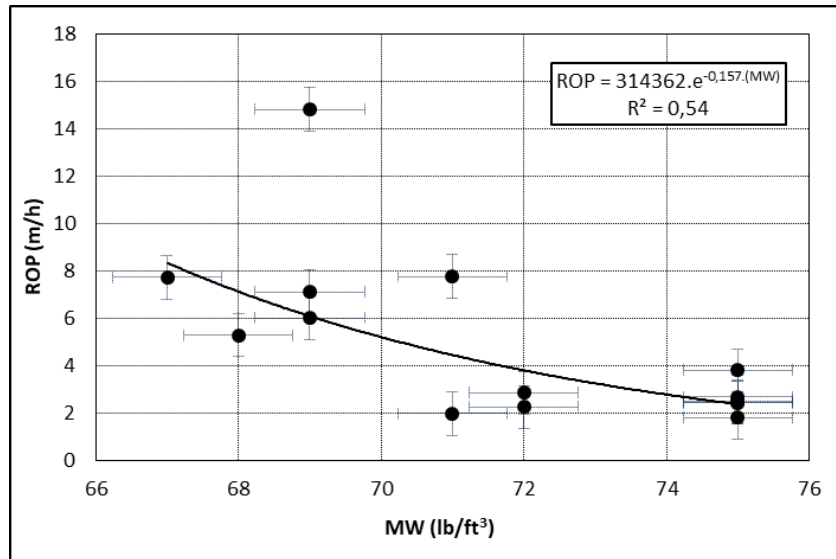
Figure 4. ROP-MW relationship diagram
