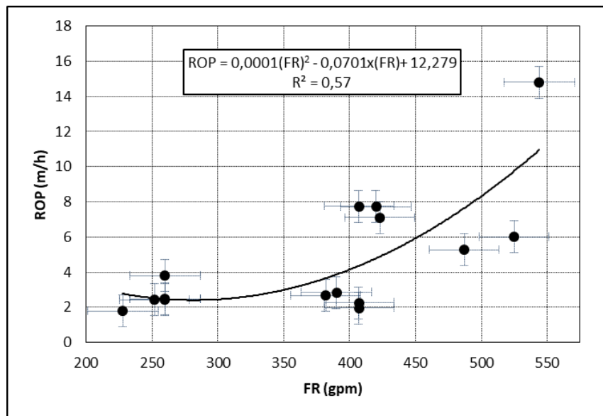
Figure 3. ROP-FR relationship diagram
