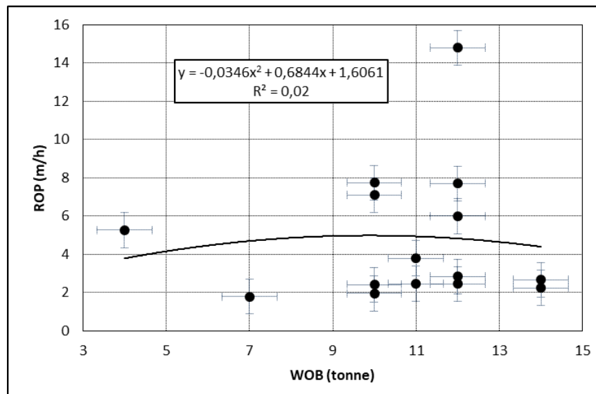
Figure 5. ROP-WOB relationship diagram
