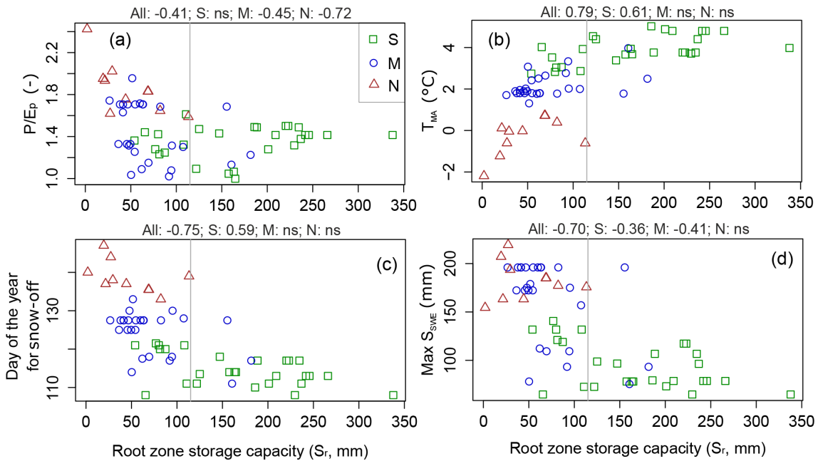
Figure 4. Root zone storage capacities and (a) ratio of average precipitation and potential evaporation ( P/E_p ), (b) mean annual temperature ( T_{MA} , °C), (c) day of the year for snow-off, and (d) maximum snow water equivalent ( S_{SWE} , mm) in the catchment at different ecoregions (S is south boreal, M is mid-boreal and N is north boreal). The titles of the sub-plots show the Spearman's correlation coefficients (significant correlation for p < 0.05 ). The line at 115 mm illustrates the discussed threshold.
